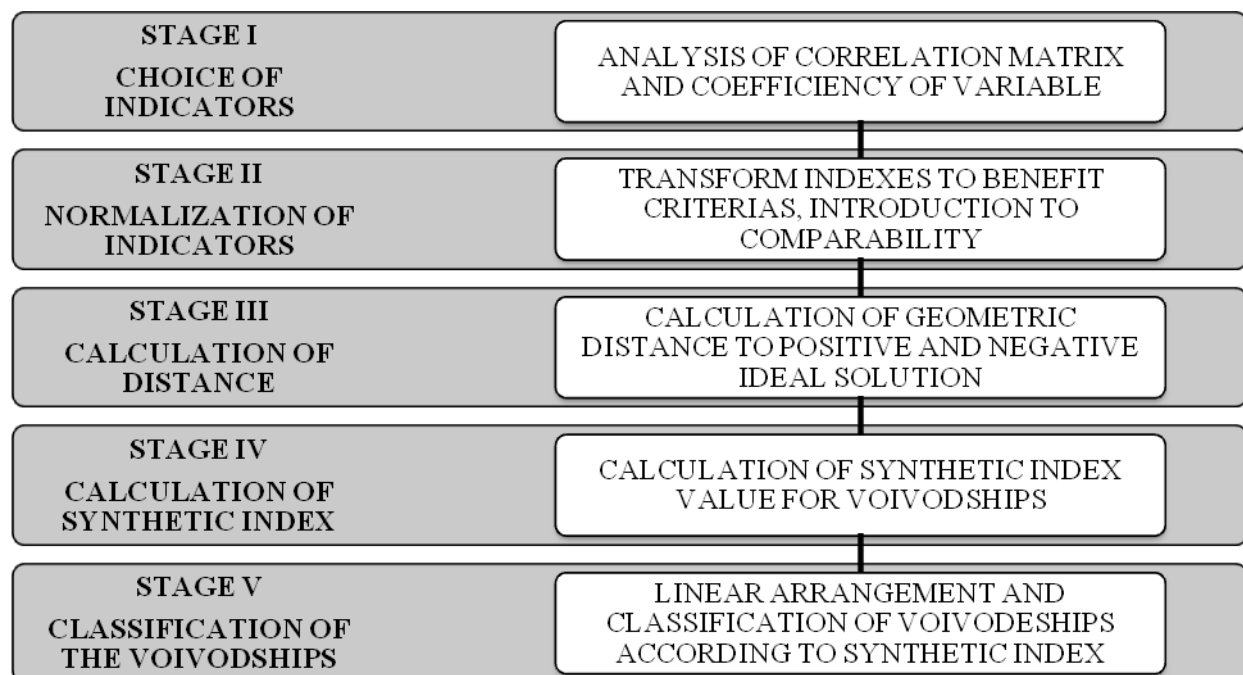
Figure 1. Diagram of the TOPSIS method
