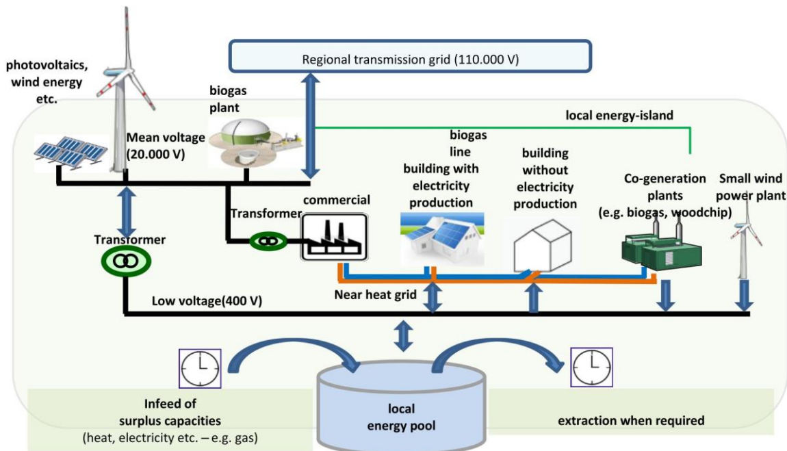
Figure 1. Local energy island
