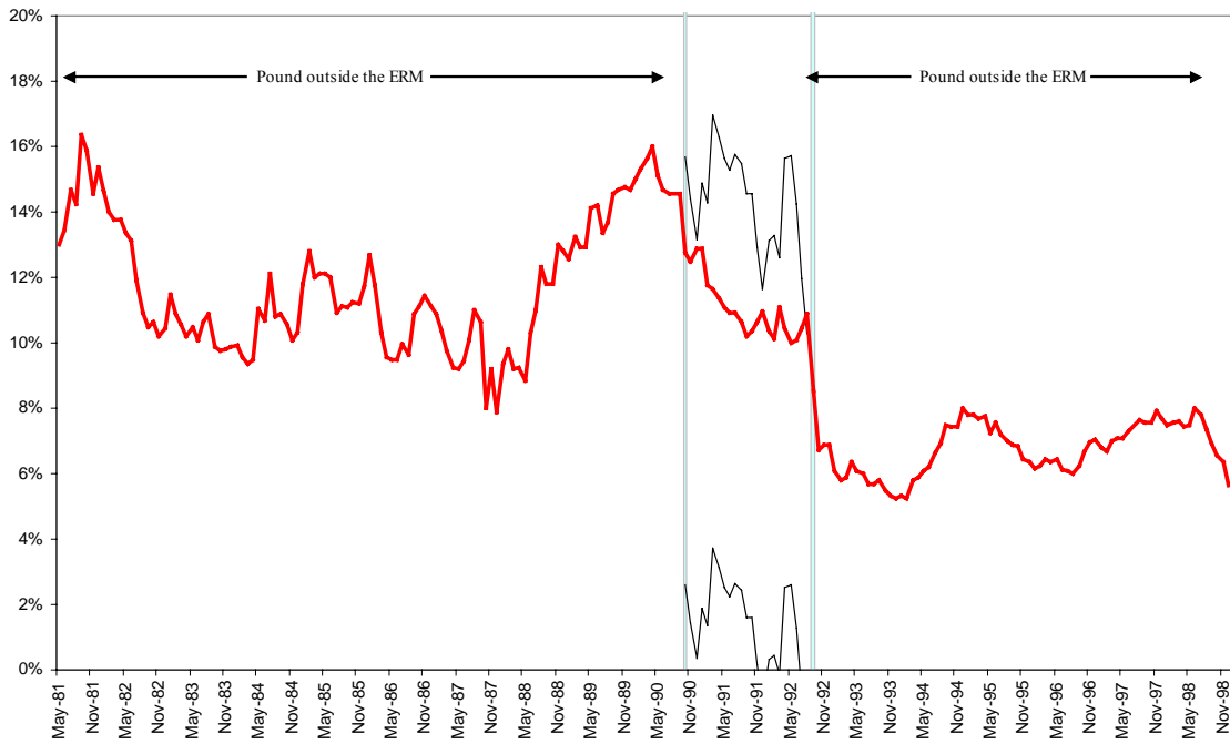
Figure 4: 12 month europound interest rate and credibility bounds
