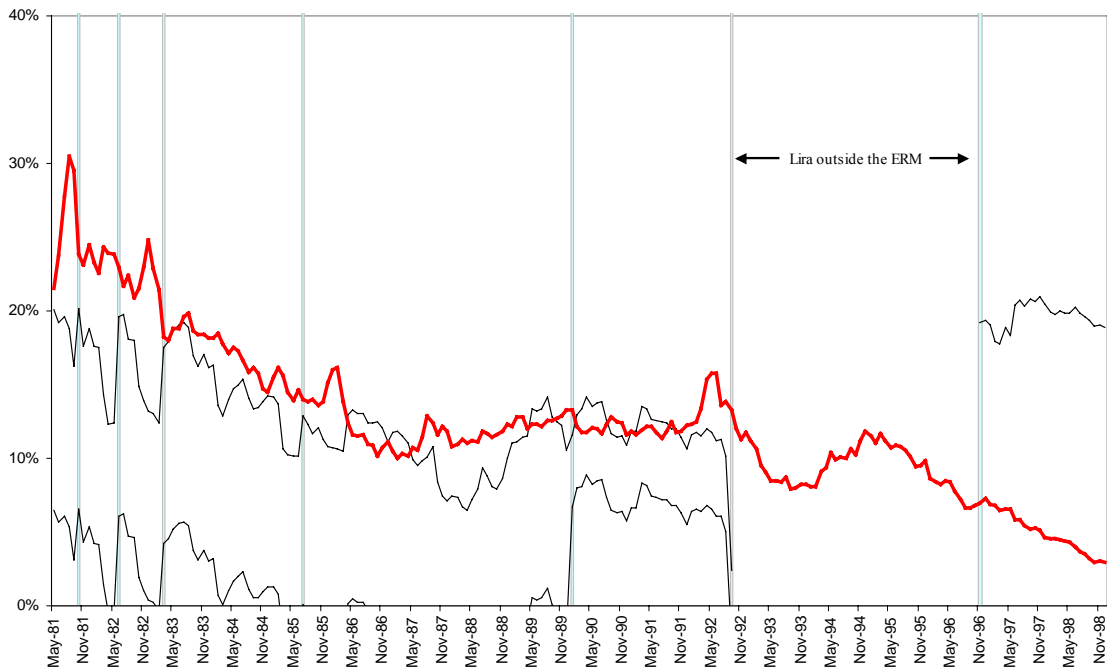
Figure 2: 12 month eurolira interest rate and credibility bounds
