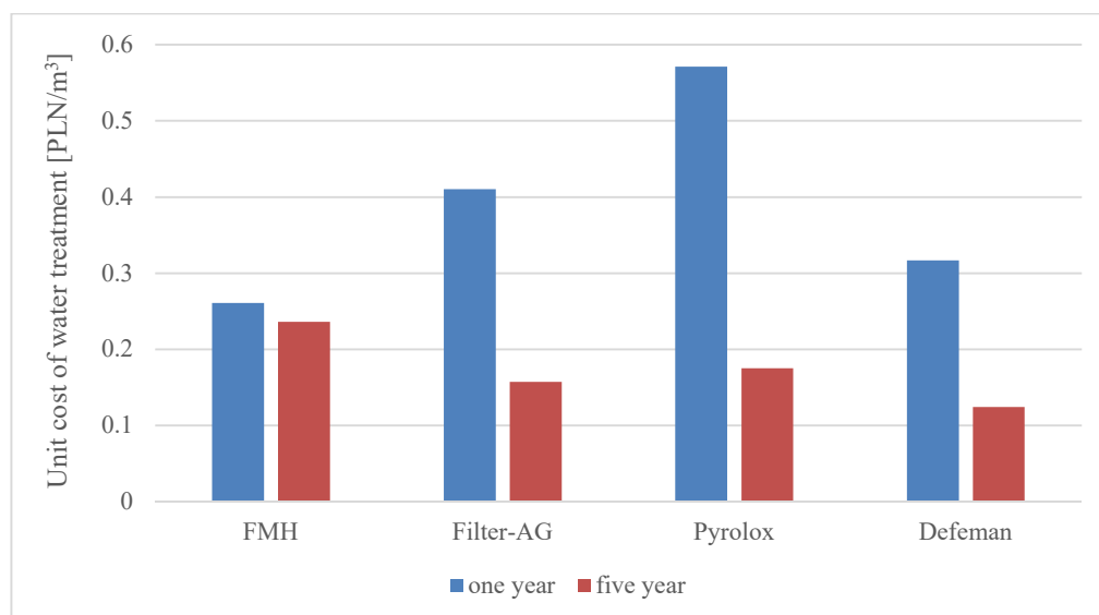
Figure 1. Summary of the unit cost of water treatment by selected filter beds
