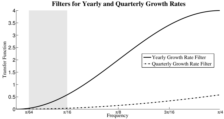
Figure 11: Comparing the Filters (1 - L^4) and (1 - L) . Note: The Figure shows the transfer functions of the yearly and quarterly growth rate filters, i.e. 2(1 - \cos(4\lambda)) and 2(1 - \cos(\lambda)) .
