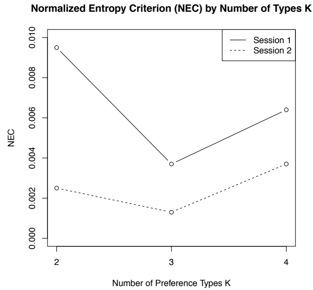
Figure S7 (Analogue to Figure 3 in the paper): Normalized entropy criterion (NEC) for different numbers of preference types in Sessions 1 and 2. The NEC summarizes the ambiguity in the subjects' classification into types relative to the finite mixture model's improvement in fit compared to the representative agent model with K = 1 (see equations 8 and 9). By minimizing the NEC, we can determine the optimal number of preference types K the finite mixture model should take into account.
