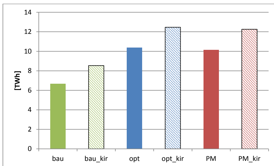
Figure 8: Net power export in 2020 per scenario
