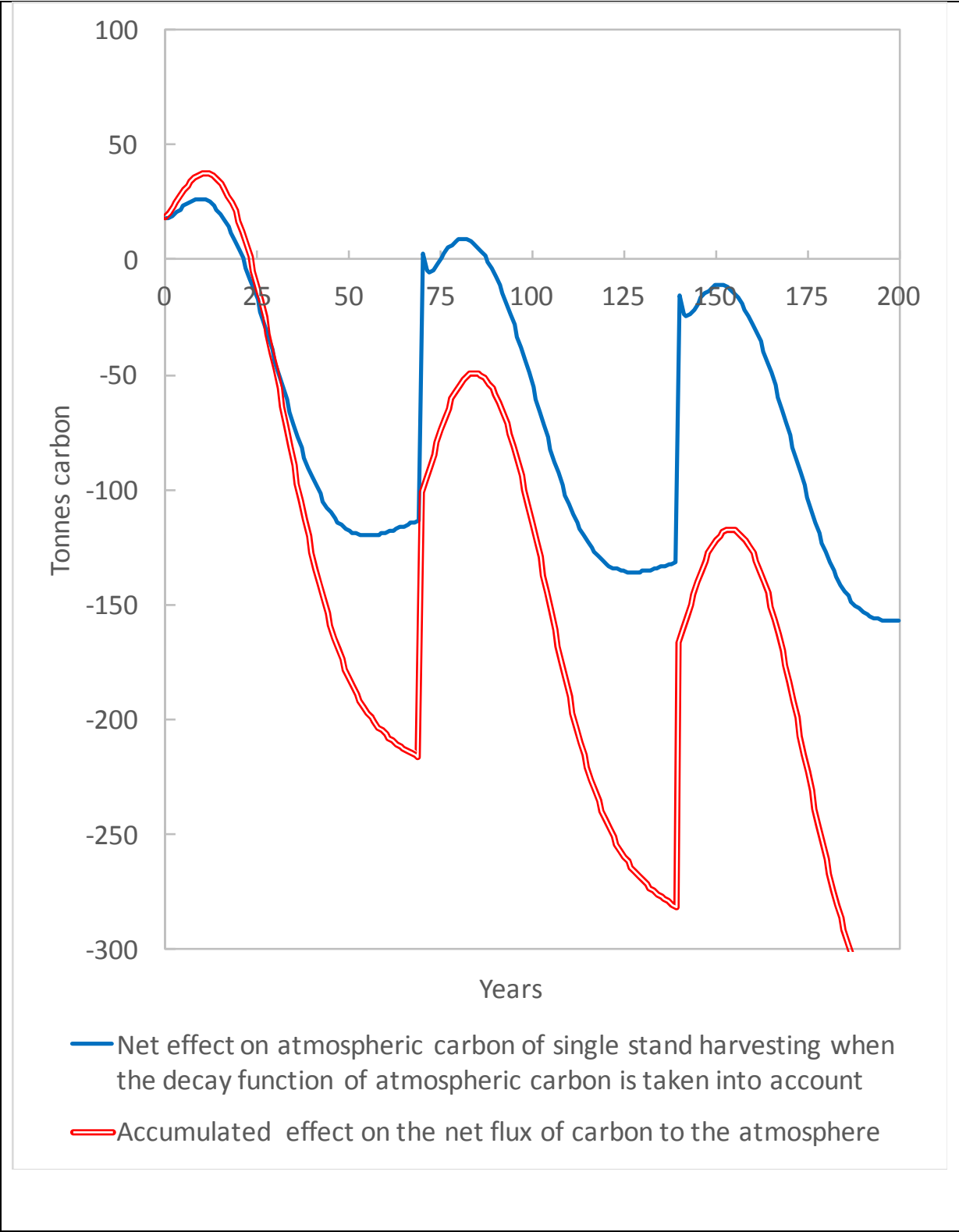
Figure 9. The blue, solid curve shows the net effect on atmospheric carbon of single stand harvesting and tree planting when the decay function of atmospheric carbon is taken into account. The red double curves shows the corresponding effect before the decay function is applied. The case with productivity indexes B20 and G20
