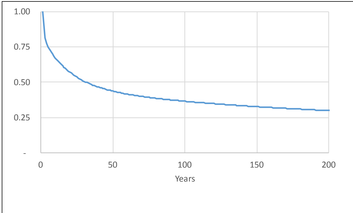
Figure 5. Share remaining in the atmosphere of a pulse of CO 2 at time 0.
