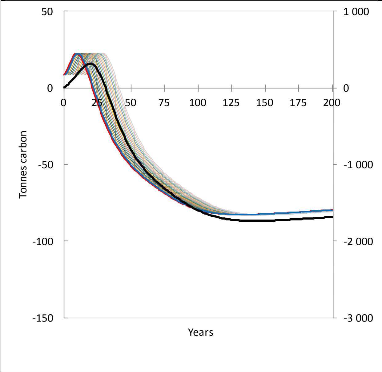
Figure 14. A scenario where bioenergy from the harvested biomass replaces 80 percent more fossil CO 2 emissions as assumed in the main cases and where harvesting of the new trees does not take place. The curves are explained in the captions to Figures 10 and 11. The case with productivity indexes B14 and G14
