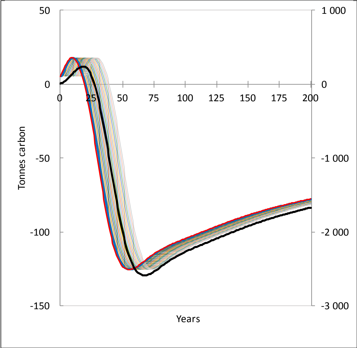
Figure 15. A scenario where bioenergy from the harvested biomass replaces 80 percent more fossil CO 2 emissions as assumed in the main cases and where harvesting of the new trees does not take place. The curves are explained in the captions to Figures 10 and 11. The case with productivity indexes B20 and G20
