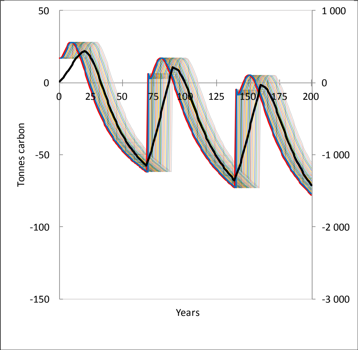
Figure 10. The red curve is the same as the blue, solid curve of Figure 8. Hence, it shows the net effect on atmospheric carbon of single stand harvesting and tree planting. The blue curve is the corresponding result of the harvesting and tree planting project taking place the subsequent year, and so forth. Hence, each of the thin curves represents each of the 20 different stands considered, respectively. These curves are measured along the left, vertical axis. The thick, black curve represents the total accumulated effect on atmospheric carbon of the 20 years program for consecutive harvesting and tree planting on the 20 stands. This accumulated, total effect is measured along the right, vertical axis. The case with productivity indexes B14 and G14
