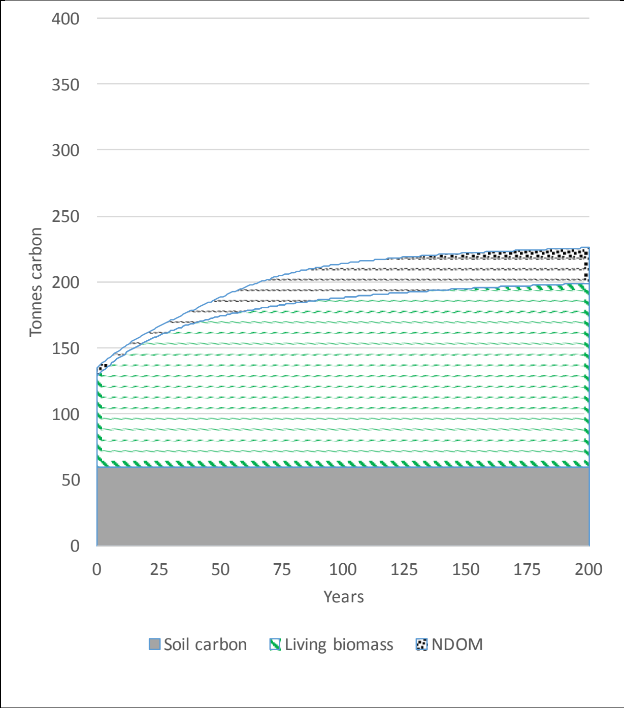
Figure 3. Development of the carbon pools of a single Birch stand in the scenario without harvesting or planting of new trees. Productivity index B20.
