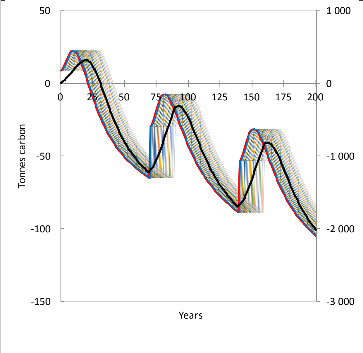
Figure 12. A scenario where bioenergy from the harvested biomass replaces 80 percent more fossil CO 2 emissions as assumed in the main cases. The curves are explained in the captions to Figures 10 and 11. The case with productivity indexes B14 and G14
