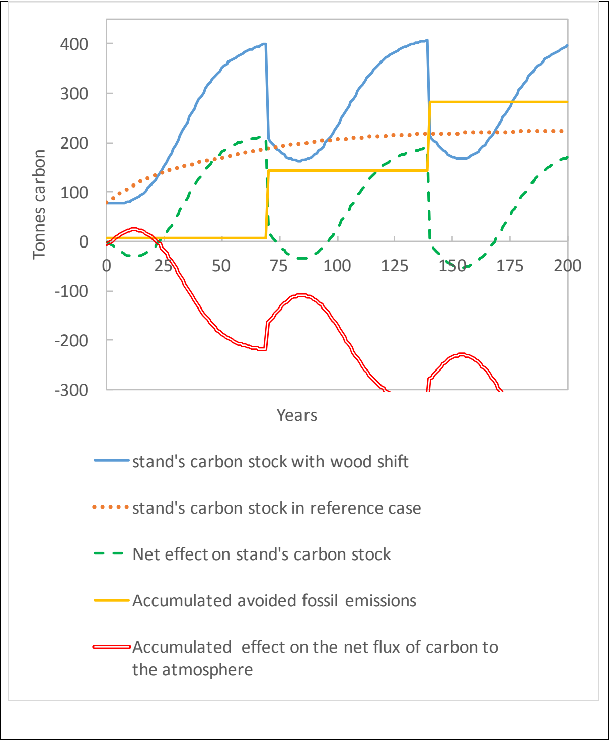
Figure 17. A case where the stand at t = 0 has 10 year old birch trees and where bioenergy from the harvested biomass replaces 80 percent more fossil CO 2 emissions as assumed in the main. Productivity index of B20 and G20
