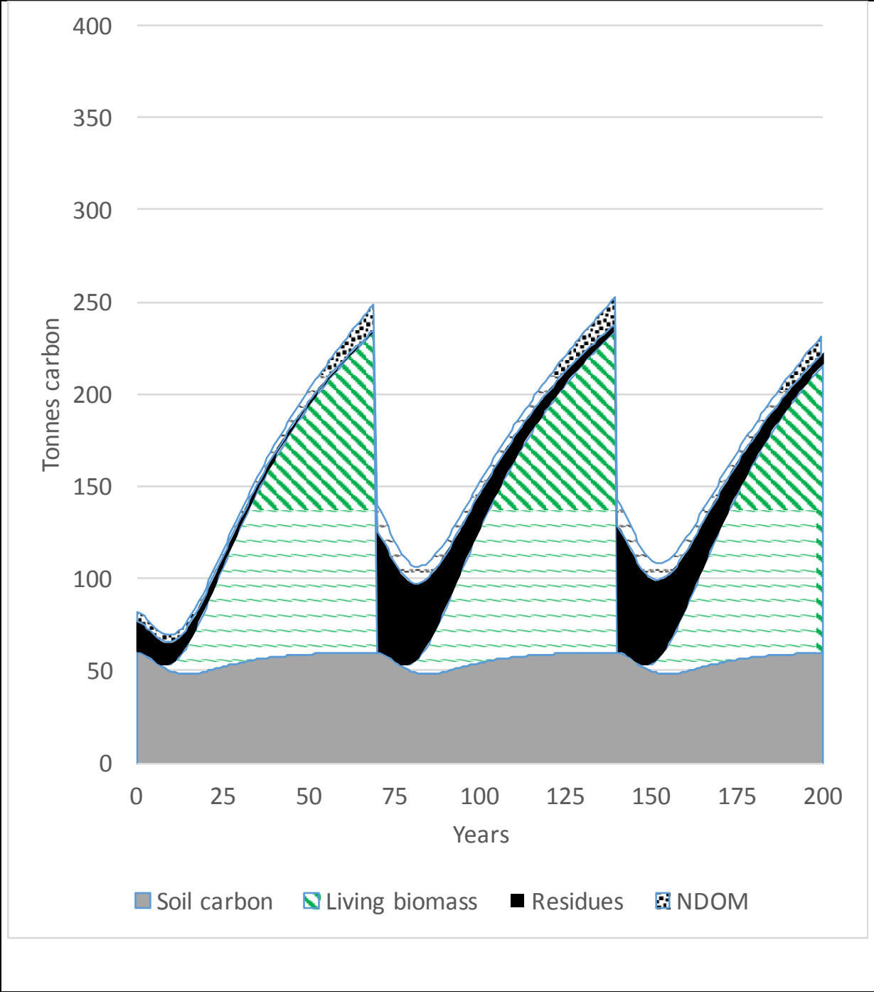
Figure 2. Development of the carbon pools of a single Spruce stand in a scenario with harvesting and tree planting. Productivity index of G14
