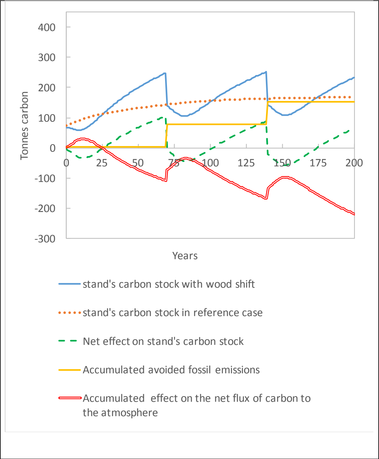
Figure 16. A case where the stand at t = 0 has 10 year old birch trees and where bioenergy from the harvested biomass replaces 80 percent more fossil CO 2 emissions as assumed in the main. Productivity index of B14 and G14
