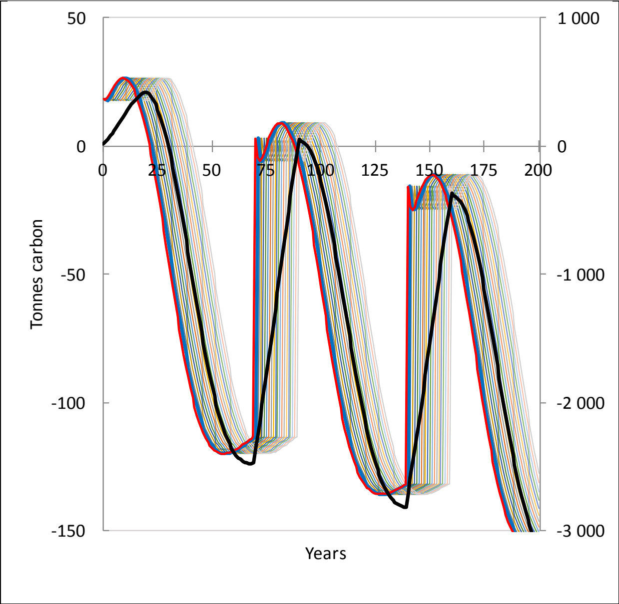
Figure 11. The red curve is the same as the blue, solid curve of Figure 9. Hence, it shows the net effect on atmospheric carbon of single stand harvesting and tree planting. The blue curve is the corresponding result of the harvesting and tree planting project taking place the subsequent year, and so forth. Hence, each of the thin curves represents the each of the 20 different stands considered, respectively. This curves are measured along the left, vertical axis. The thick, black curve represents the total accumulated effect on atmospheric carbon of the 20 years program for harvesting and tree planting on new areas and is measured along the right, vertical axis. The case with productivity indexes B20 and G20
