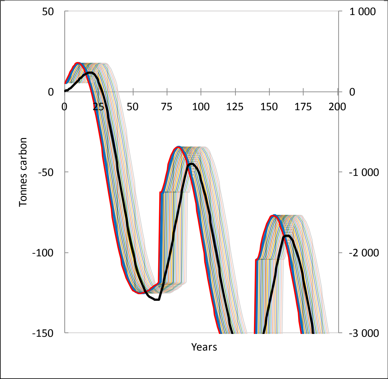
Figure 13. A scenario where bioenergy from the harvested biomass replaces 80 percent more fossil CO 2 emissions as assumed in the main cases. The curves are explained in the captions to Figures 10 and 11. The case with productivity indexes B20 and G20
