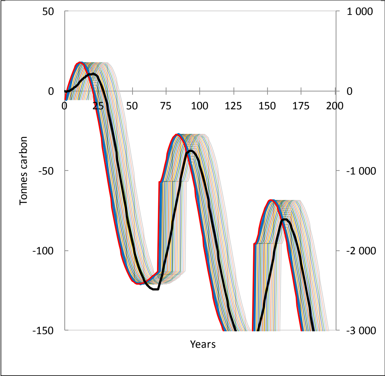
Figure 19. A case where the stand at t=0 has 10 year old birch trees and where bioenergy from the harvested biomass replaces 80 percent more fossil CO 2 emissions as assumed in the main.
