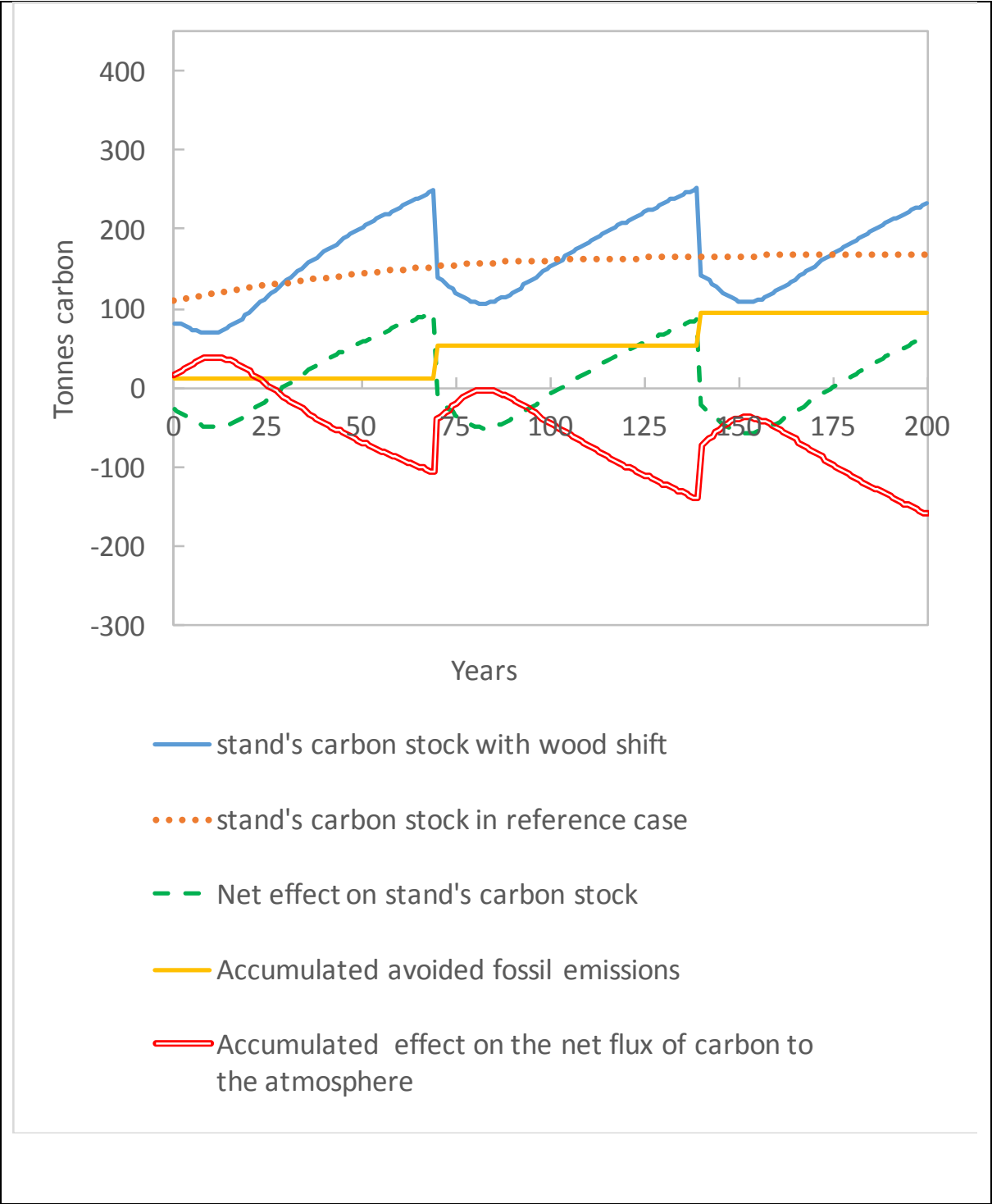
Figure 6. Development of the considered stand's carbon stock in both the reference scenario and the harvesting and tree planting scenario together with avoided accumulated fossil carbon emissions and the accumulated effect on the net flux of carbon to the atmosphere. Productivity index of B14 and G14
