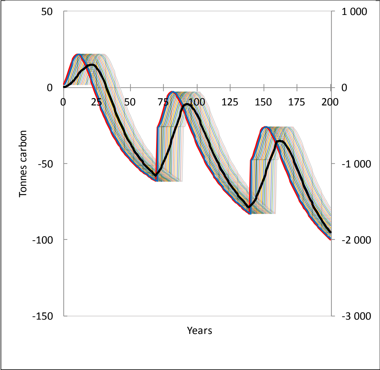
Figure 18. A case where the stand at t = 0 has 10 year old birch trees and where bioenergy from the harvested biomass replaces 80 percent more fossil CO 2 emissions as assumed in the main.
