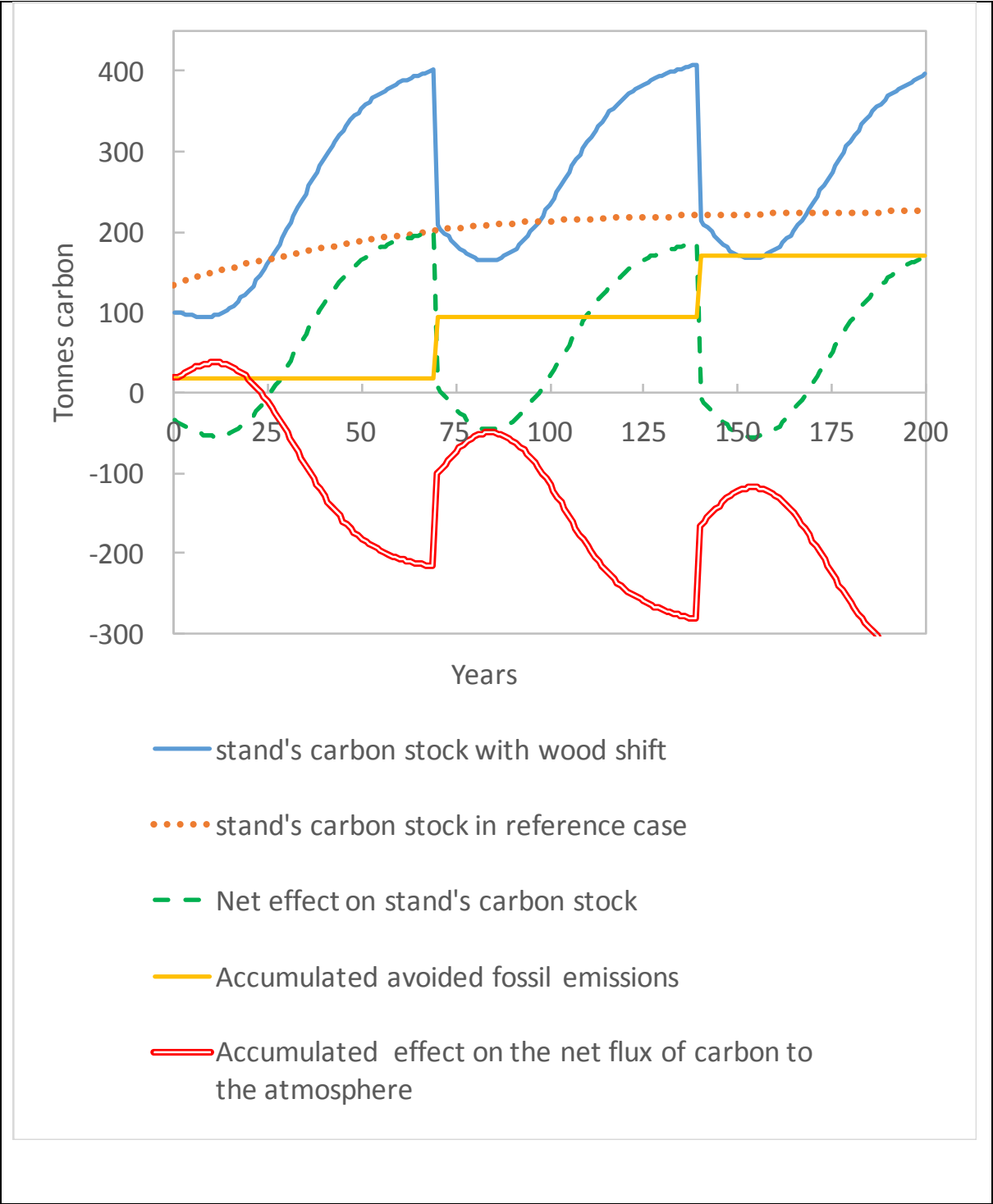
Figure 7. Development of the considered stand's carbon stock in both the reference scenario and the harvesting and tree planting scenario together with avoided accumulated fossil carbon emissions and the accumulated effect on the net flux of carbon to the atmosphere. Productivity index of B20 and G20
