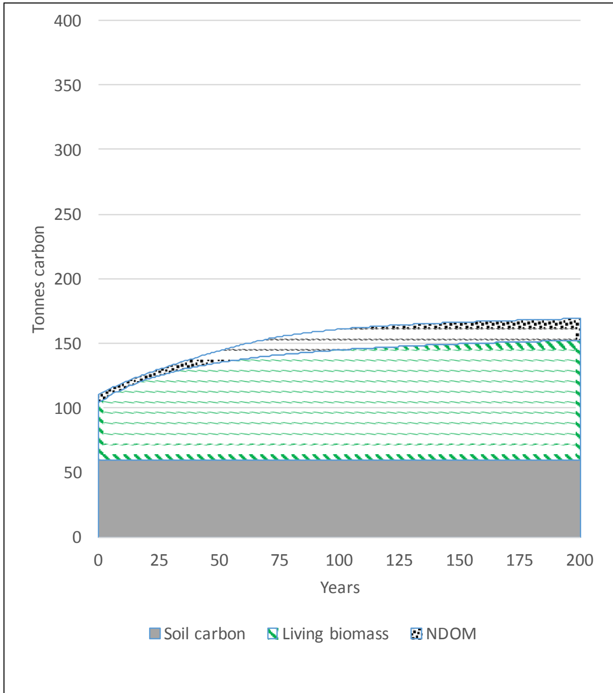
Figure 1. Development of the carbon pools of a single Birch stand in the scenario without harvesting or planting of new trees. Productivity index B14.
