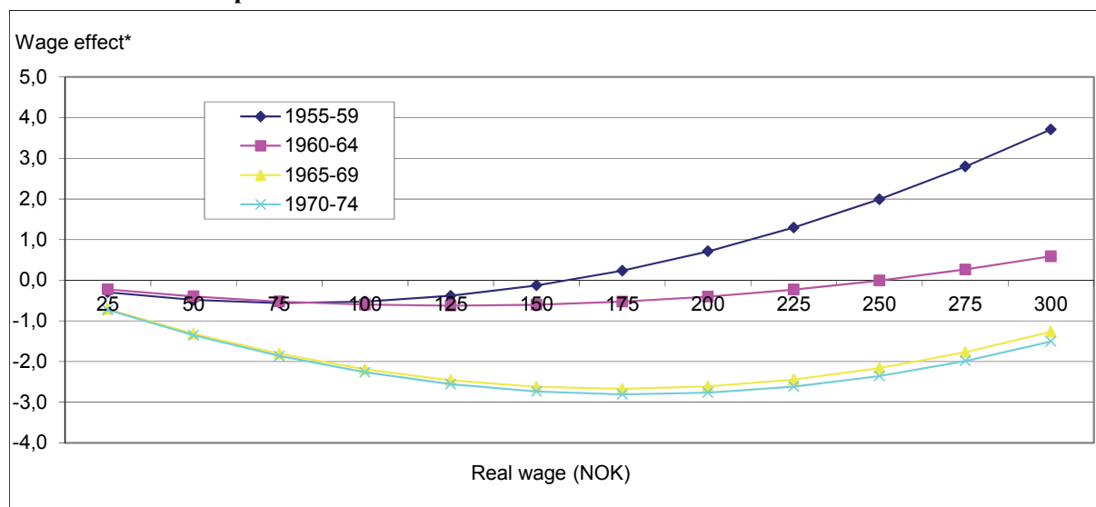
Figure B3. The shape of the wage effect on log hazard for the third birth, for four different cohorts. Specifications with education variables
