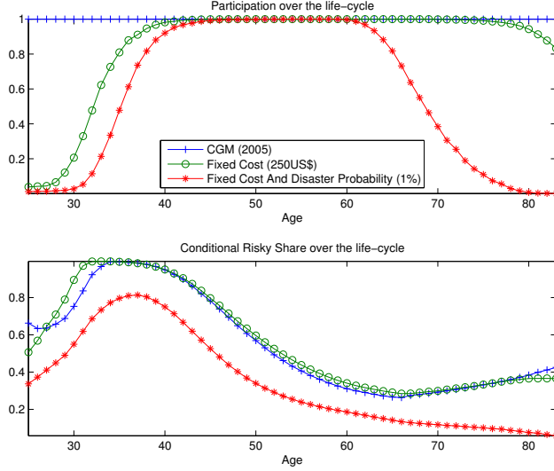
Figure 6.3: Model Simulation
