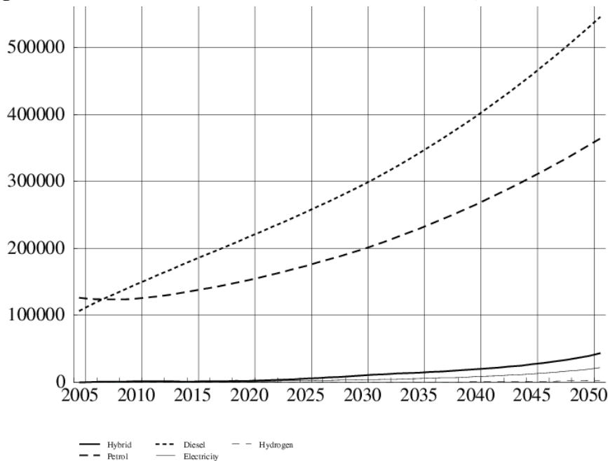
Figure 4.3. The stock of cars in the uniform tax scenario, mill 2004-NOK
