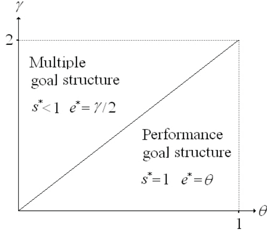
Figure 2: Equilibria in the static framework
