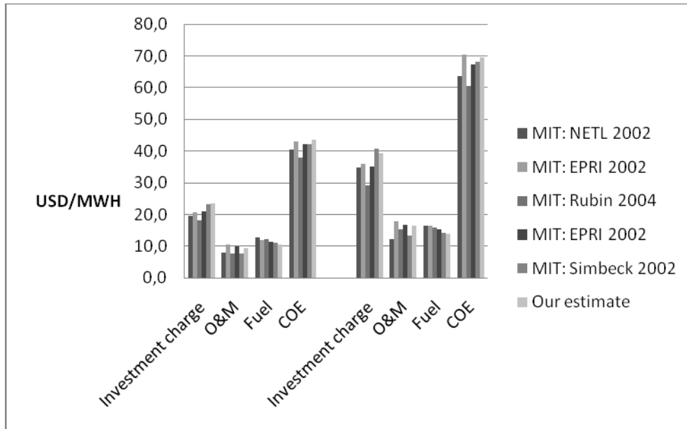
Figure A1 LIBEMOD PC estimates compared to “normalized” studies in MIT report (first four clusters of columns are without CCS, last four with CCS)
