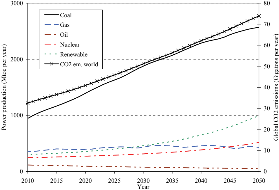
Figure 1. Global power production (Mtoe) from different technologies and global CO 2 emissions (Gigatons) per year. Reference scenario
