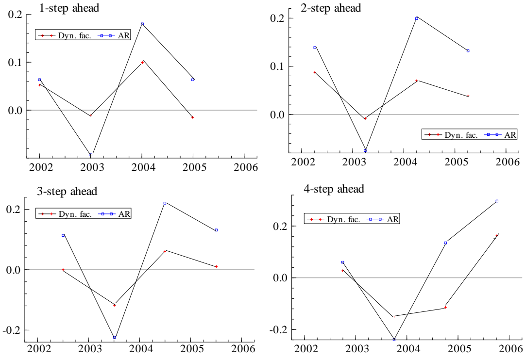
Figure 1: Forecasting errors at different horizons for INVM (log scale)
