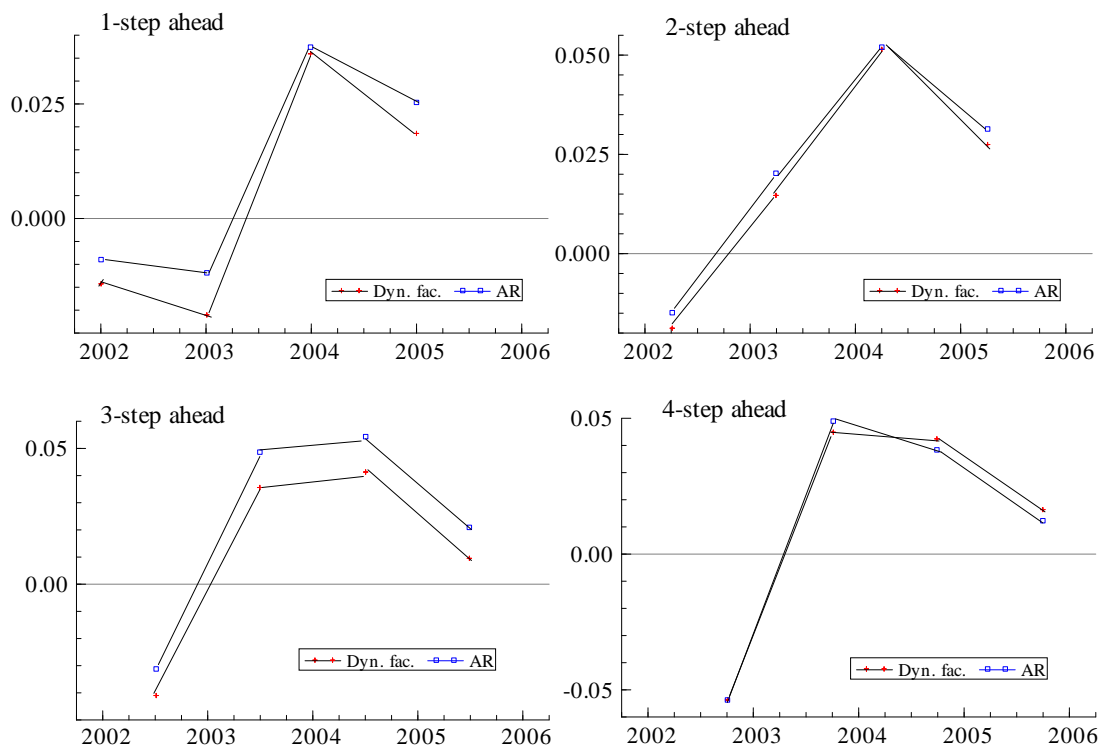
Figure 3: Forecast errors at different horizons for PRIM: Benchmark AR vs. DFM(5,3) (log scale)
