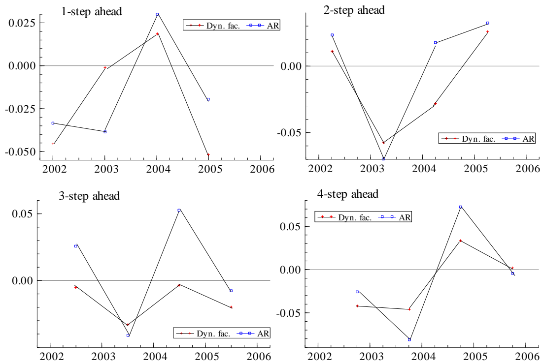
Figure 2: Forecasts errors at different horizons for MM: Benchmark AR vs. DFM(5,3) (log scale)
