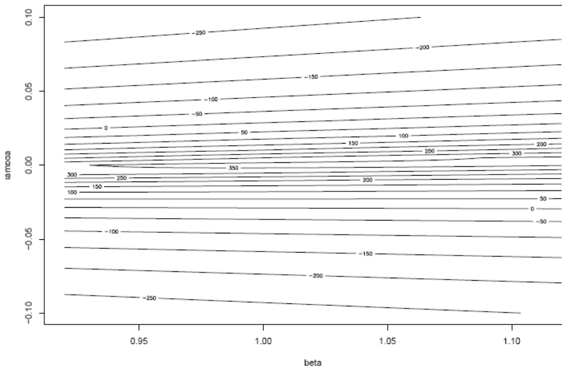
Figure A1. European data. Concentrated log likelihood for the baseline model. Contour plot
