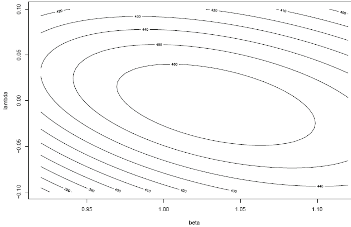
Figure A3. US data. Concentrated log likelihood for the baseline model. Contour plot
