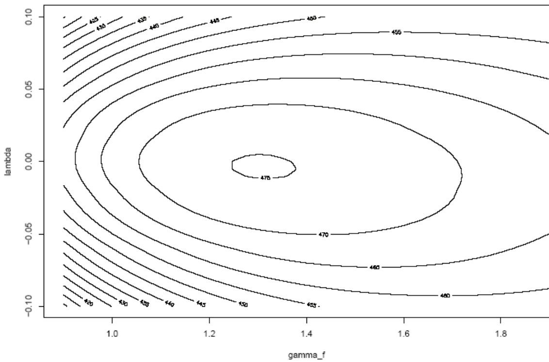
Figure A4. US data. Concentrated log likelihood for the hybrid model. Contour plot
