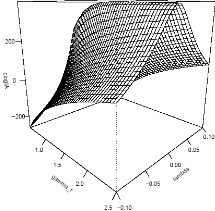
Figure 3. Concentrated log likelihood for the hybrid model. Surface plot
