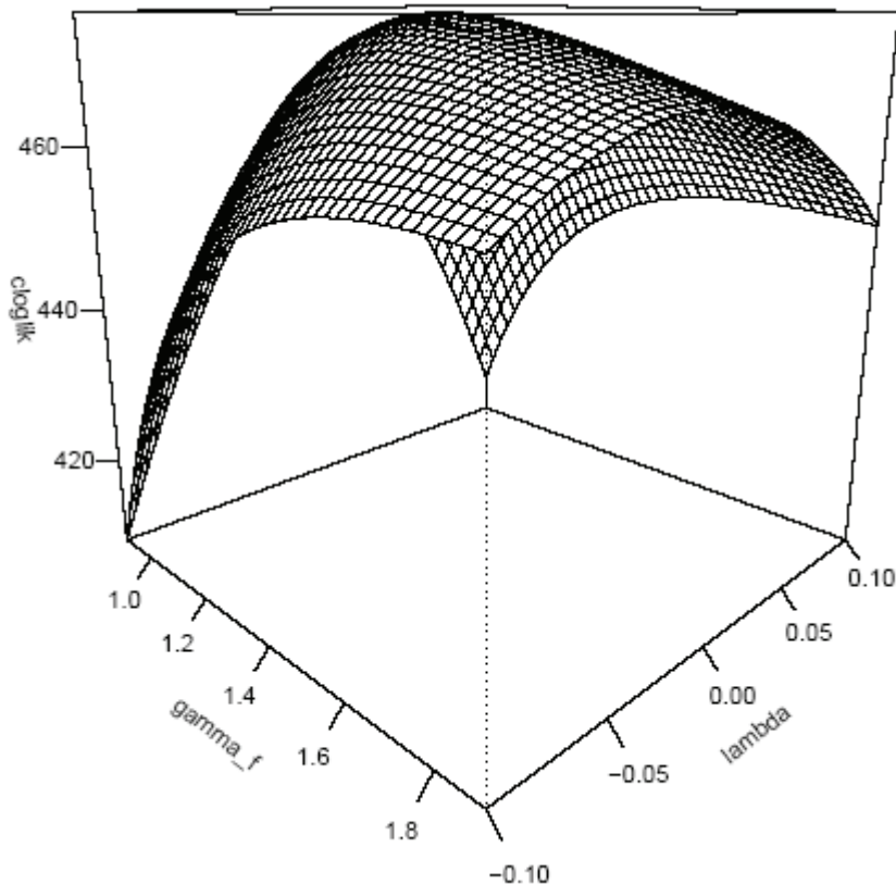
Figure 6. Concentrated log likelihood for the hybrid model. Surface plot
