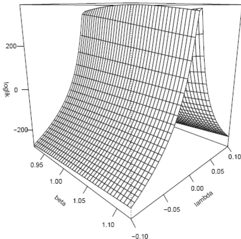
Figure 2. Concentrated log likelihood for the baseline model. Surface plot
