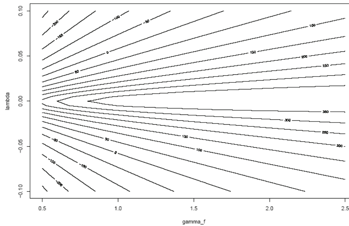
Figure A2. European data. Concentrated log likelihood for the hybrid model. Contour plot
