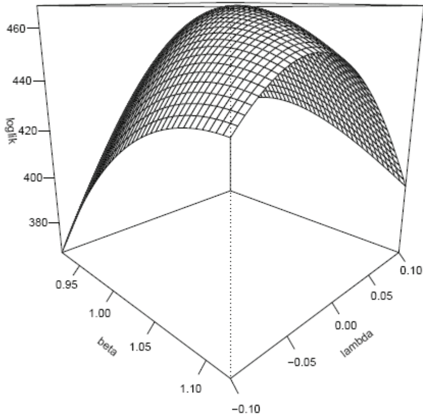
Figure 5. Concentrated log likelihood for the baseline model. Surface plot
