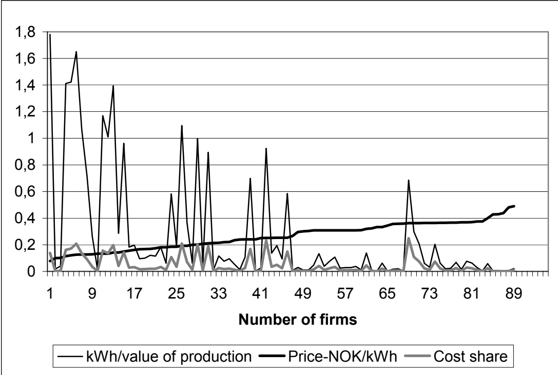
Figure 3.2 The price of electricity, the electricity input coefficient and the cost share by firm. Chemical industry
