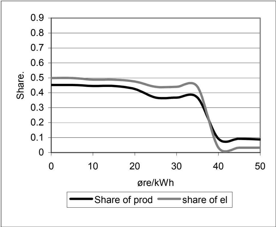
Figure 3.4 Electricity and production share of total as the minimum electricity price increase and a sufficient long term surplus is presupposed. Pulp and paper industry
