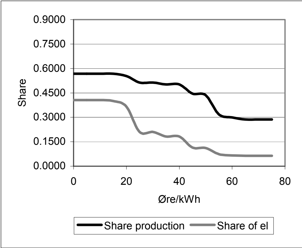
Figure 3.5 Electricity and production share of total as the minimum electricity price increase and sufficient long term surplus is presupposed. Chemical industry
