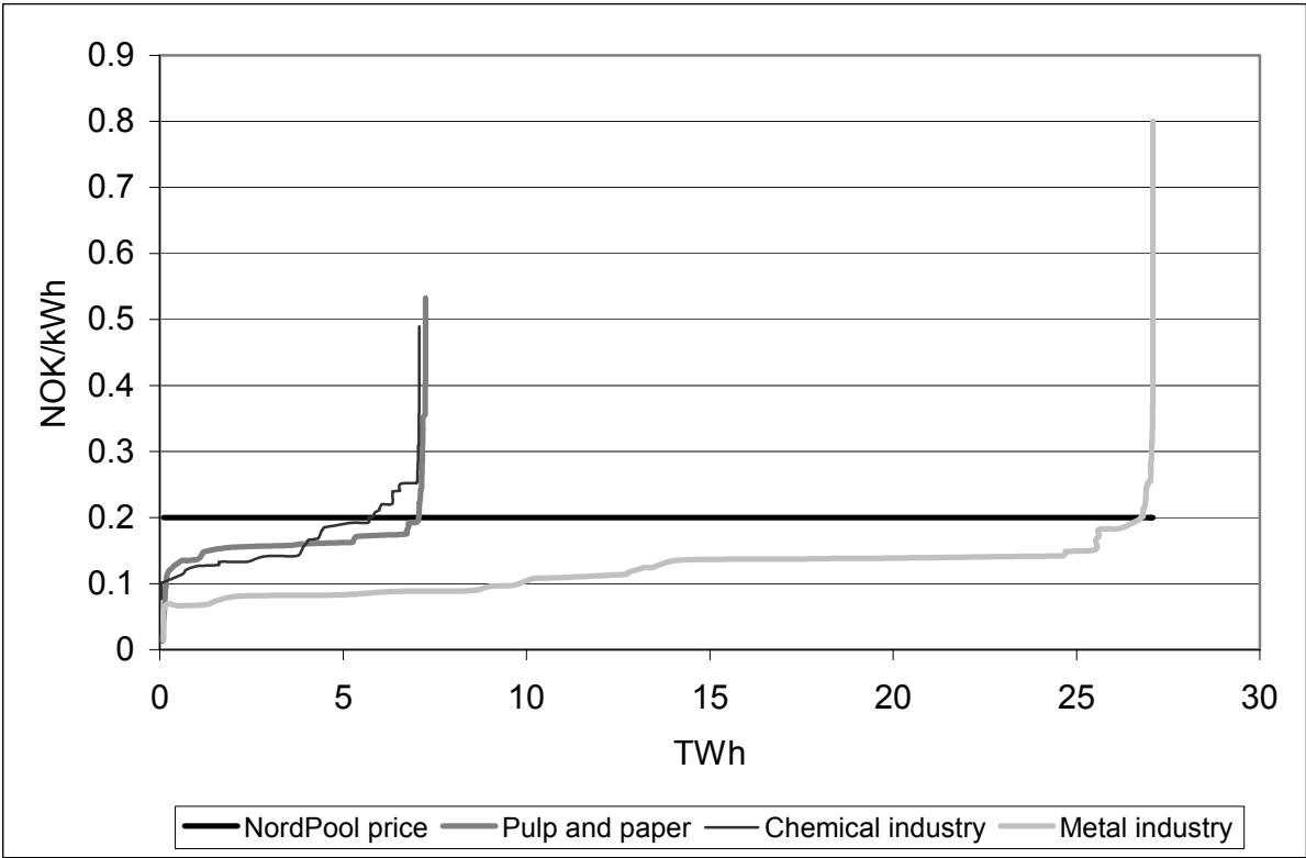
Figure 2.1. Price and volume of electricity in the pulp and paper industri, the chemicals industry and the metals industry. The market price at NordPool. TWh and NOK/kWh. 2000
