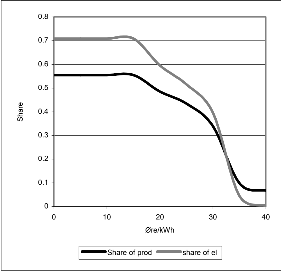
Figure 3.6 Electricity and production share of total as the minimum electricity price increase and a sufficient long term surplus is presupposed. Metal industry
