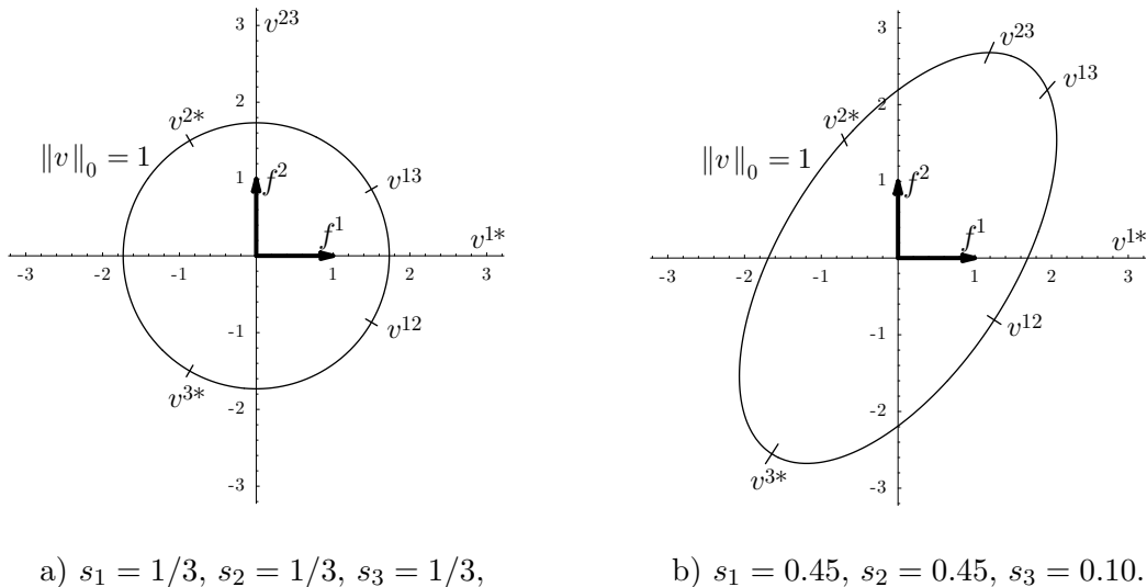
Figure 2: The unit spheres of two elasticity metrics
