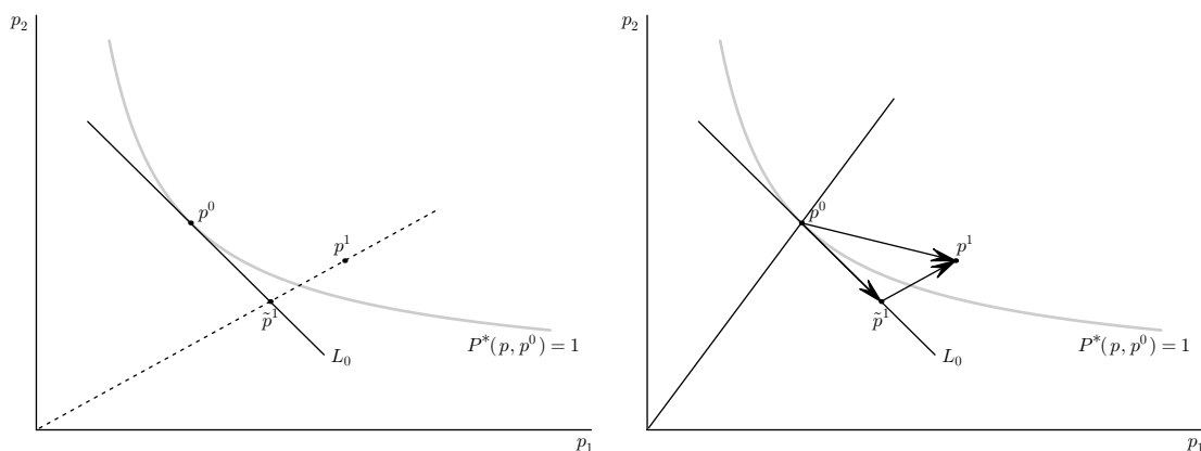
a) Deflating onto the Laspeyres plane, b) Decomposition of the price change.
