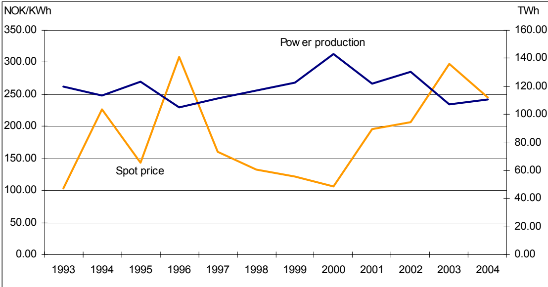
Figure 2. The spot price (NOK/kWh left axis) and hydro power production (TWh-right axis)
