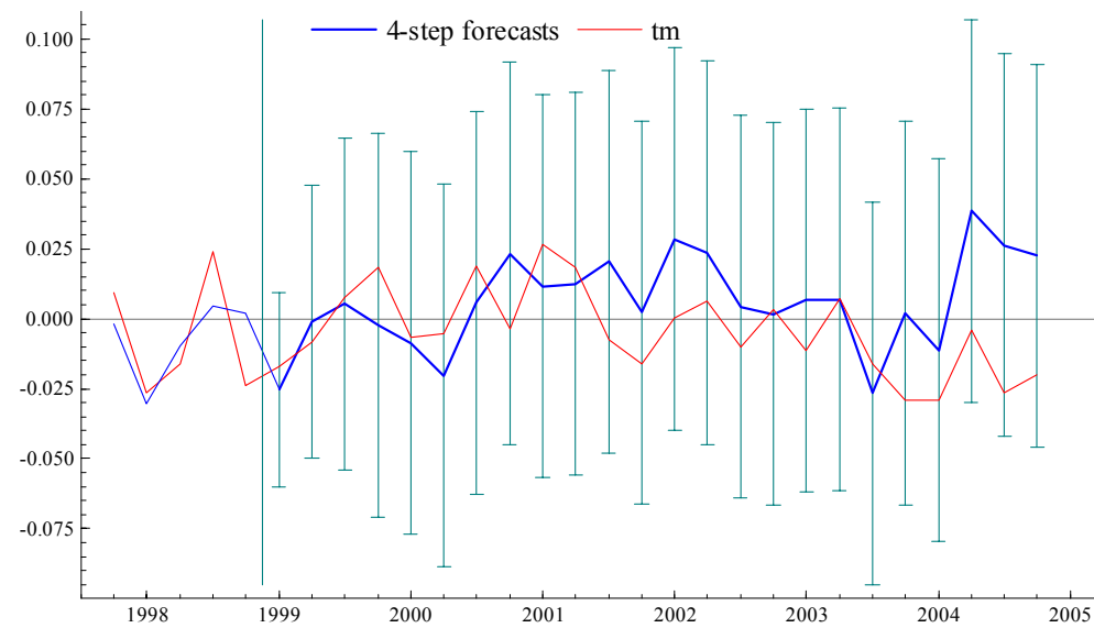
Figure 2b. Actual values of tm_t and 4-step ahead forecasts with 95 % bands
