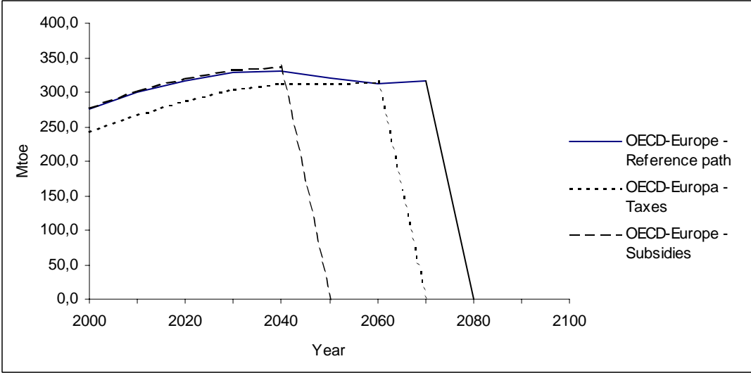
Figure 8: Gas production in OECD-Europe
