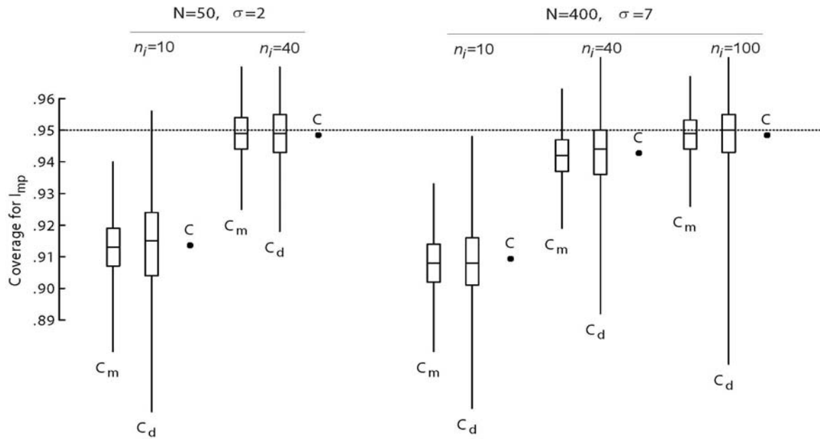
Figure 6. Box-plots of 1000 C_d - and C_m estimates for I_{mp} with \beta = 1, \mu = 3, \tau = 1, \rho = .5 .
