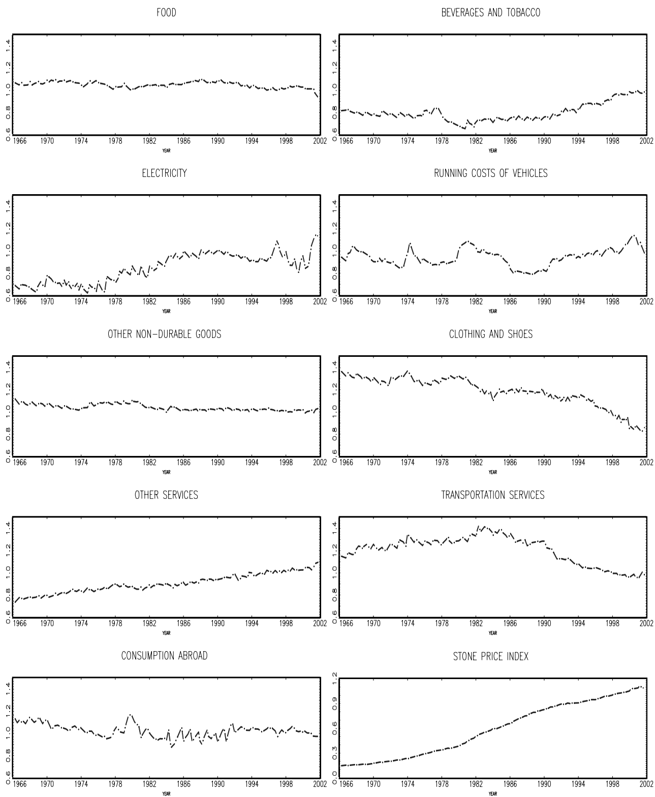
Figure 2: Deflated prices P_{jt}/P_t^* and the Stone price index, P_t^* .
