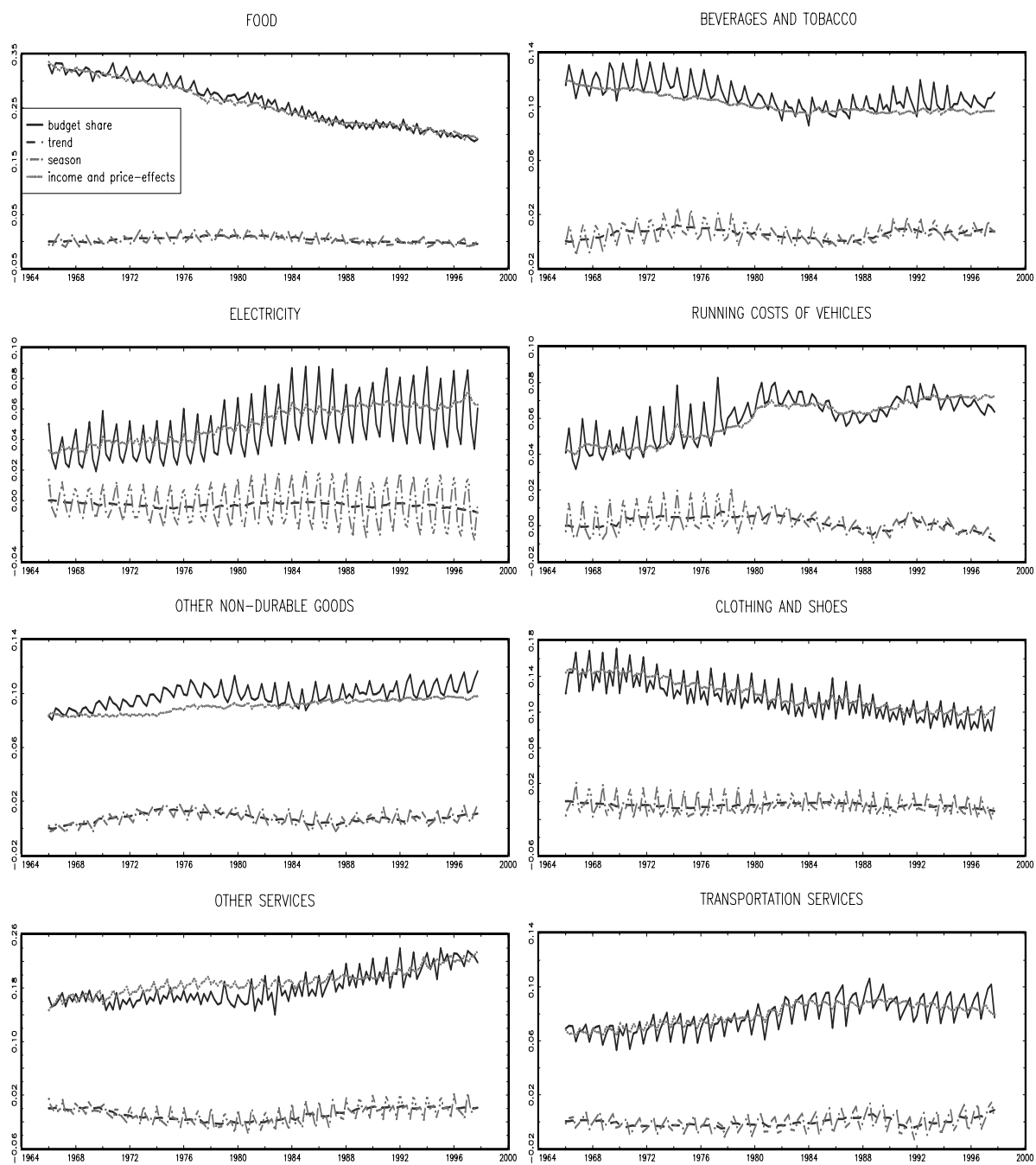
Figure 4: Non-homogeneous model: Actual budget shares versus trend, season, and income/price effects
