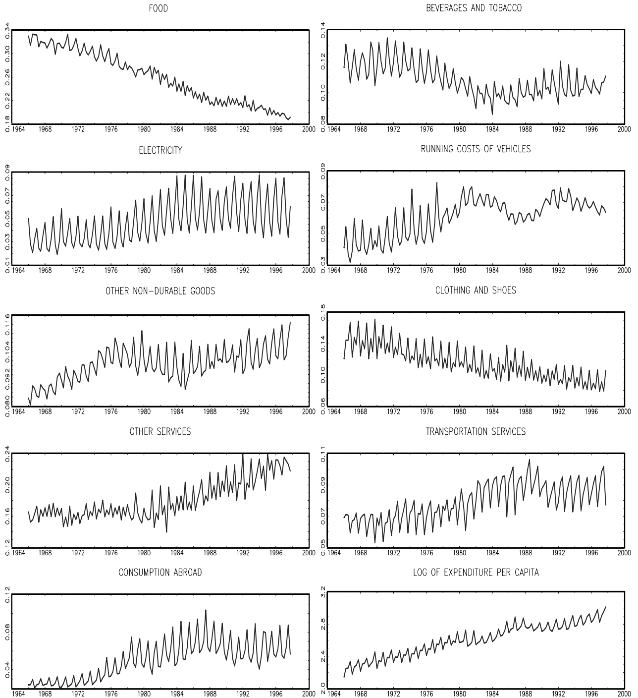
Figure 1: Budget shares and log of total expenditure per capita
