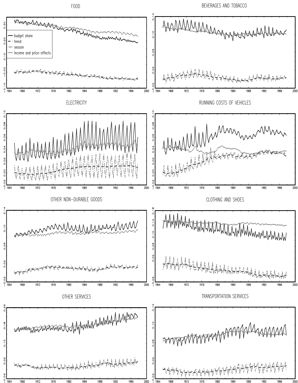
Figure 3: Homogeneous model: Actual budget shares versus trend, season, and income/price effects
