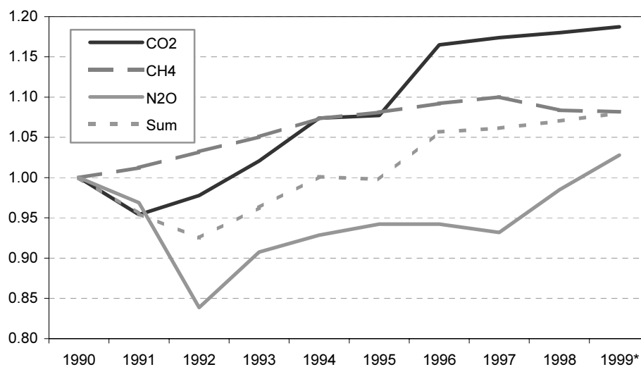
Figure 1. GHG emissions in Norway 1990–1999, 1990=1. CO 2 , methane, N 2 O and sum 1)
