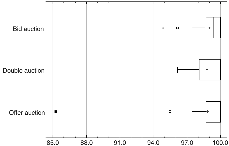
Figure 3. Efficiency levels, by auction type
