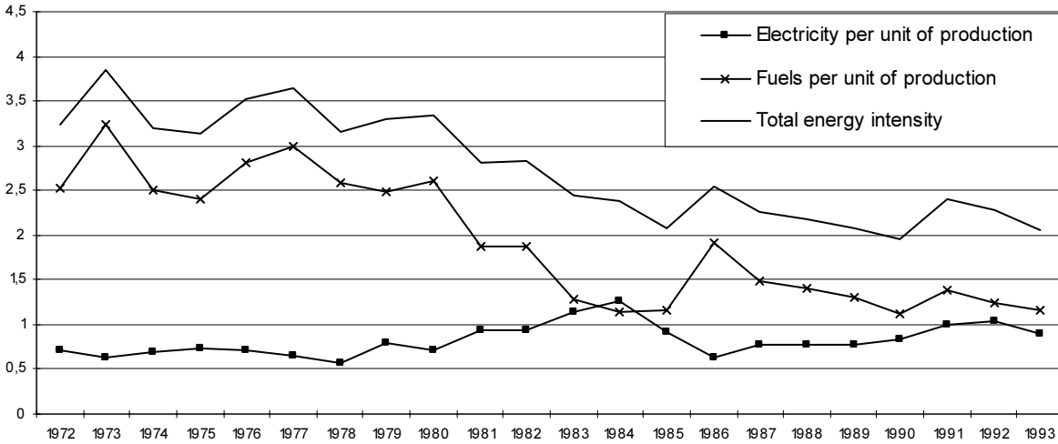
Figure 3.5. Energy intensity in the production of cellulose, MWh/ton
