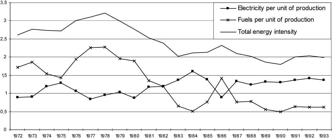
Figure 3.7. Energy intensity in the production of paper, MWh/ton
