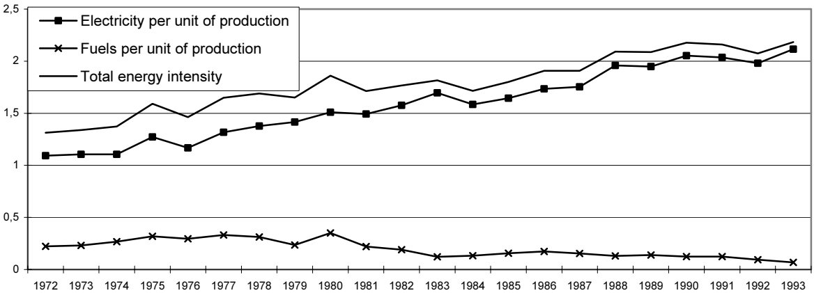
Figure 3.3. Energy intensity in the production of mechanical pulp, MWh/ton
