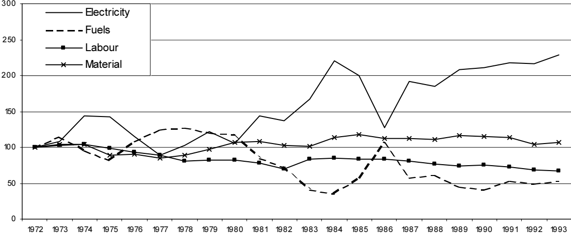
Figure 3.6. Use of inputs in the paper production, 1972=100
