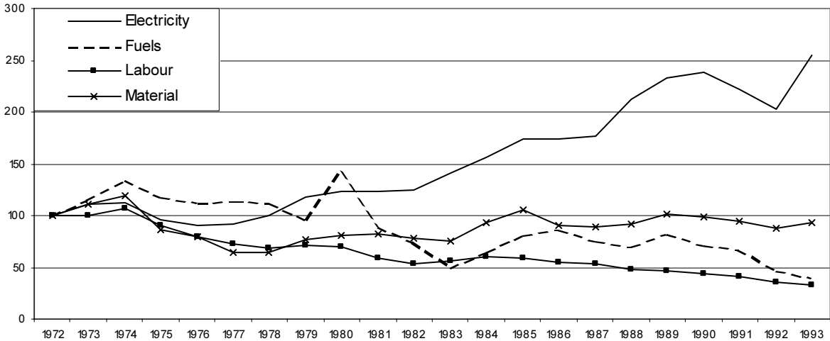
Figure 3.2. Use of inputs in the production of mechanical pulp, 1972=100
