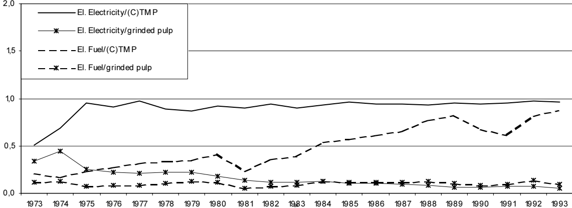
Figure 4.1. Output elasticity for the mechanical pulp producers
