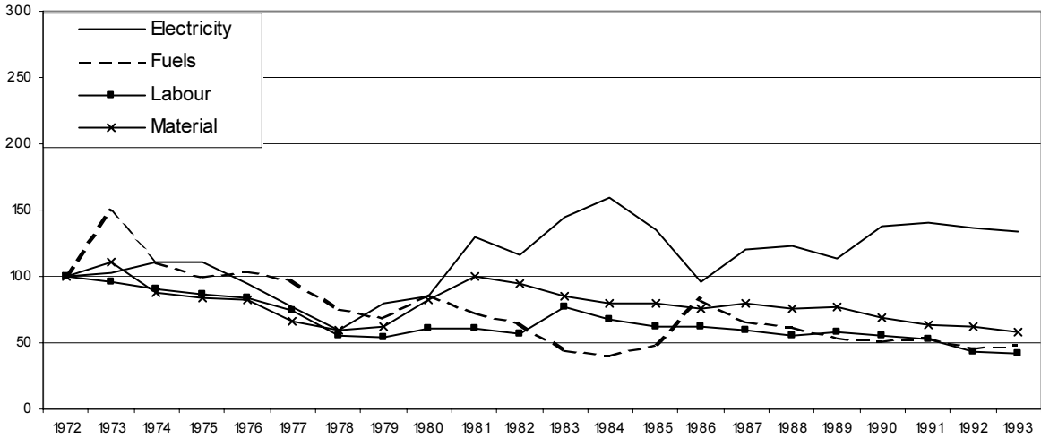
Figure 3.4. Use of inputs in the production of cellulose, 1972=100
