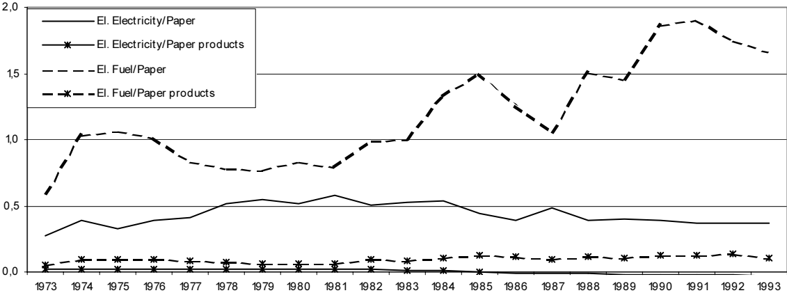
Figure 4.3. Output elasticity for the paper producers
