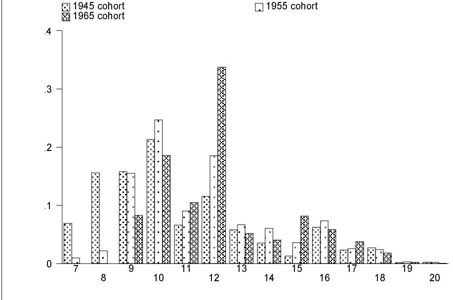
Figure 2: Distribution of years of schooling for selected cohorts. 1997
