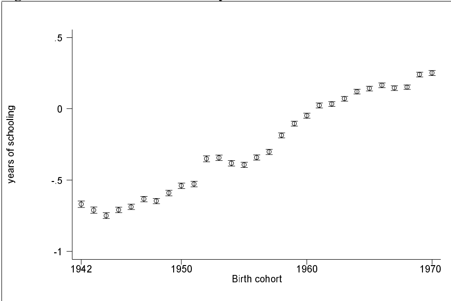
Figure 3: Educational attainment by cohort. Partial female effect
