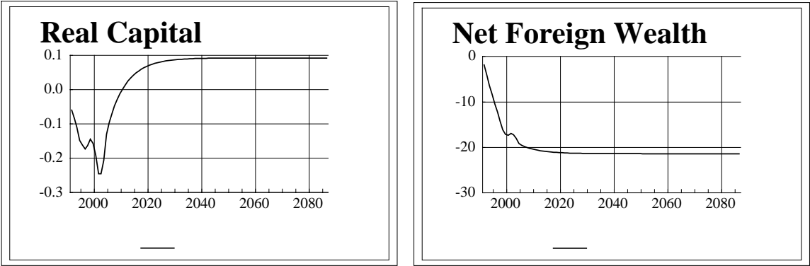
Figure 3: Equilibrium dynamics of real capital and net foreign wealth, percentage deviations between the post- and pre-reform scenarios
