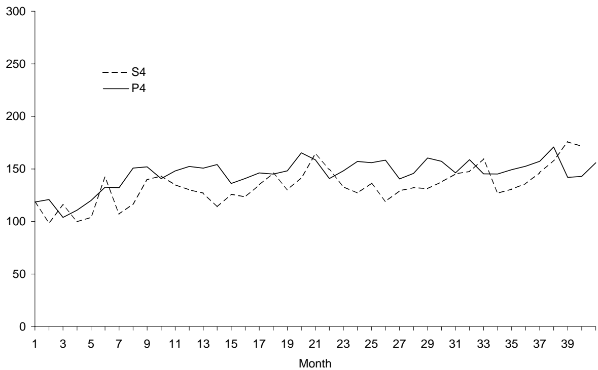
Figure 4. Plot of S_{4t} and (EP_{i4t}^{\alpha_4})^{1/\alpha_4}
