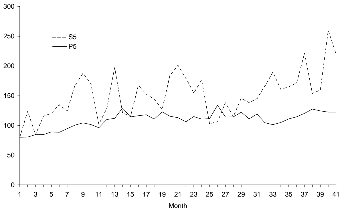
Figure 5. Plot of S_{5t} and (EP_{i5t}^{\alpha_5})^{1/\alpha_5}
