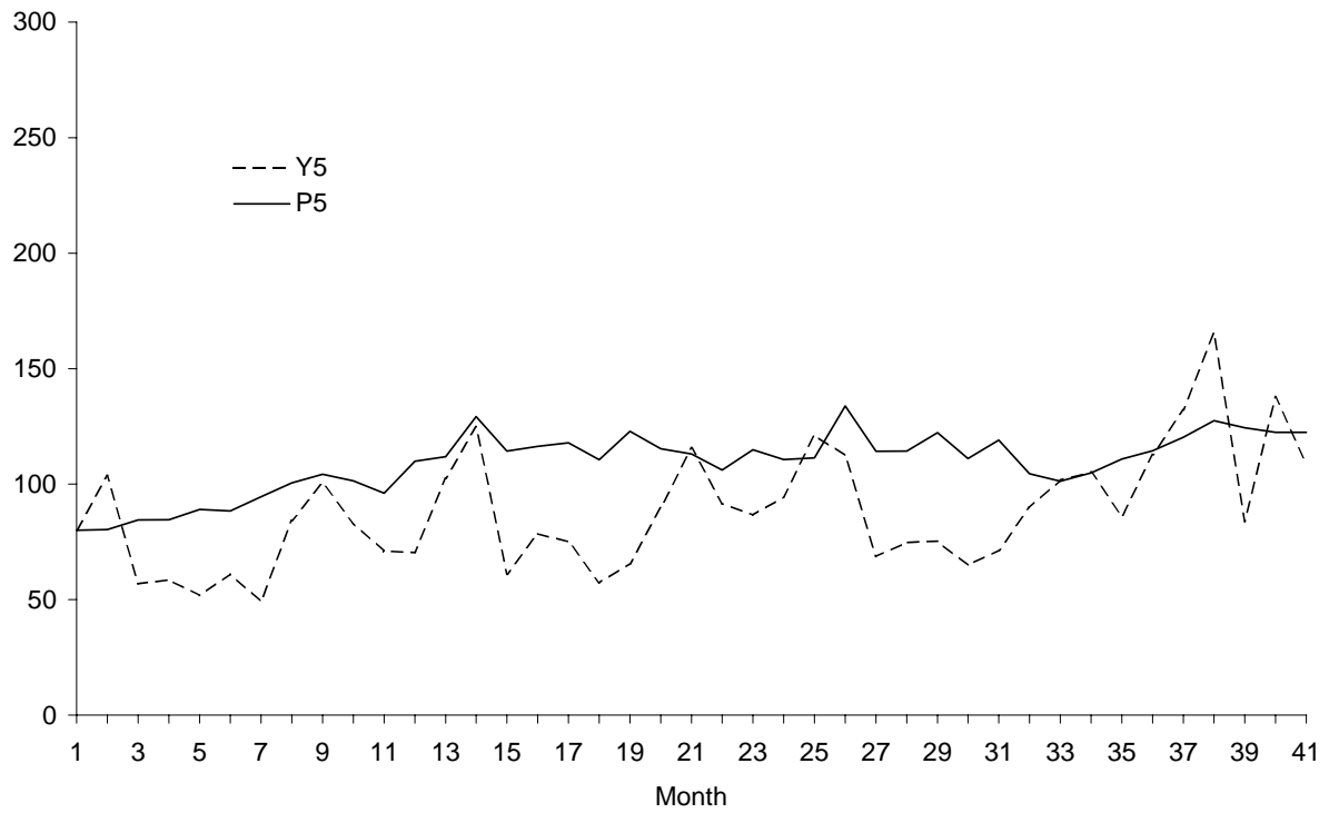
Figure 11. Plot of \bar{y}_{5t} and (\hat{EP}_{i5t}^{\alpha_5})^{1/\alpha_5}
