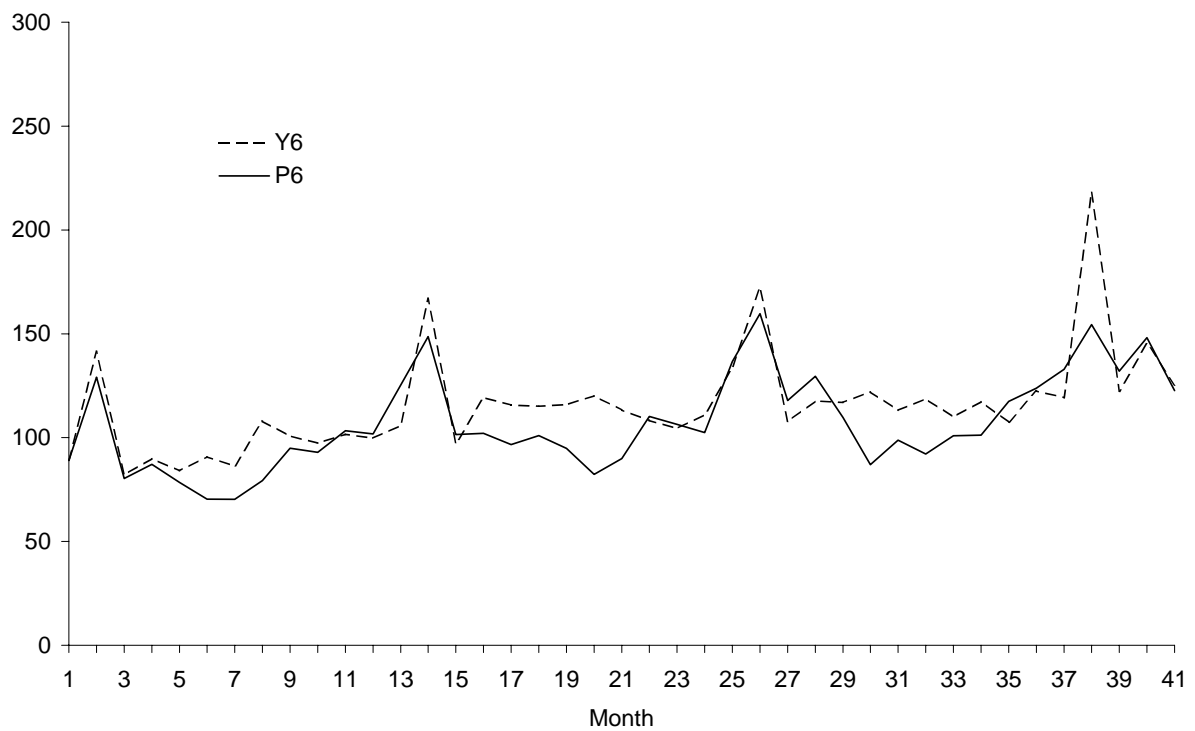
Figure 12. Plot of \bar{y}_{6t} and (\hat{EP}_{i6t}^{\alpha_6})^{1/\alpha_6}
