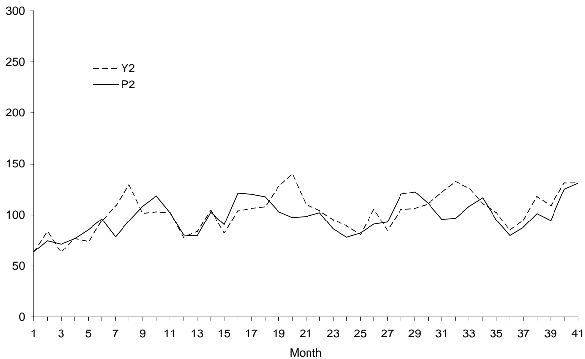
Figure 8. Plot of \bar{y}_{2t} and (EP_{2t}^{\alpha_2})^{1/\alpha_2}
