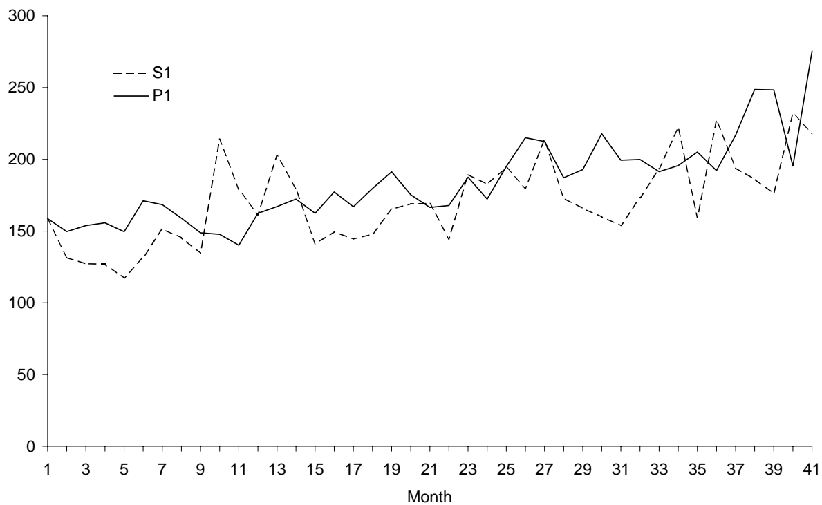
Figure 1. Plot of S_{1t} and (\hat{E}P_{1t}^{\alpha_1})^{1/\alpha_1}
