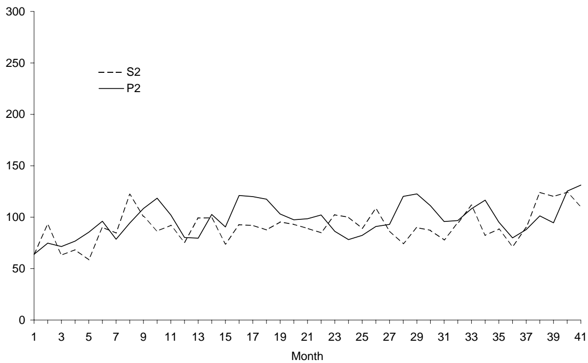
Figure 2. Plot of S_{2t} and (\hat{E}P_{2t}^{\alpha_2})^{1/\alpha_2}
