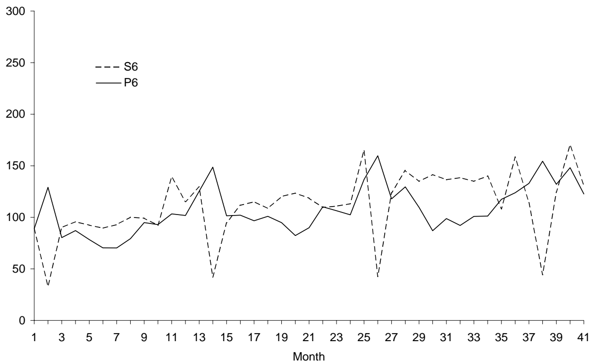
Figure 6. Plot of S_{6t} and (EP_{i6t}^{\alpha_6})^{1/\alpha_6}
