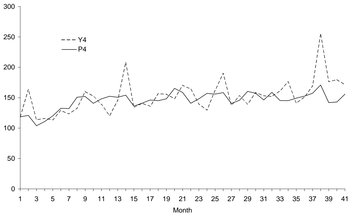
Figure 10. Plot of \bar{y}_{4t} and (E\hat{P}_{i4t}^{\alpha_4})^{1/\alpha_4}
