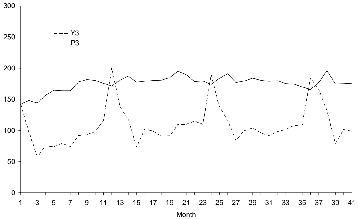
Figure 9. Plot of \bar{y}_{3t} and (E\hat{P}_{i3t}^{\alpha_3})^{1/\alpha_3}
