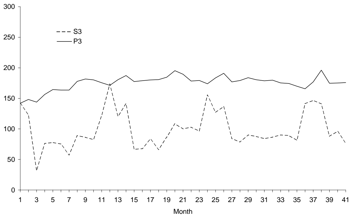
Figure 3. Plot of S_{3t} and (EP_{i3t}^{\alpha_3})^{1/\alpha_3}
