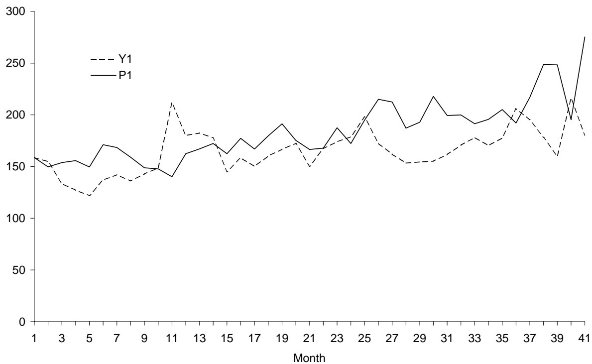
Figure 7. Plot of \bar{y}_{1t} and (EP_{1t}^{\alpha_1})^{1/\alpha_1}
