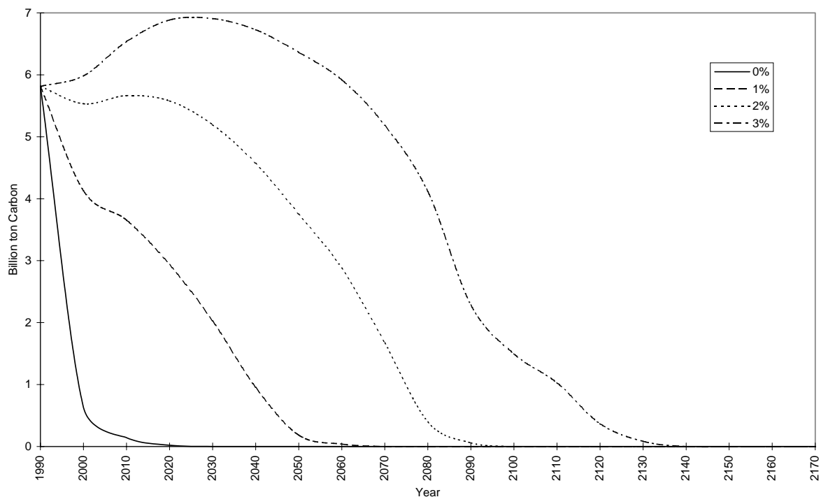
Figure 4.4. Sensitivity analyses on the pure rate of time preference (CAT2). Global carbon emissions (billion tons)
