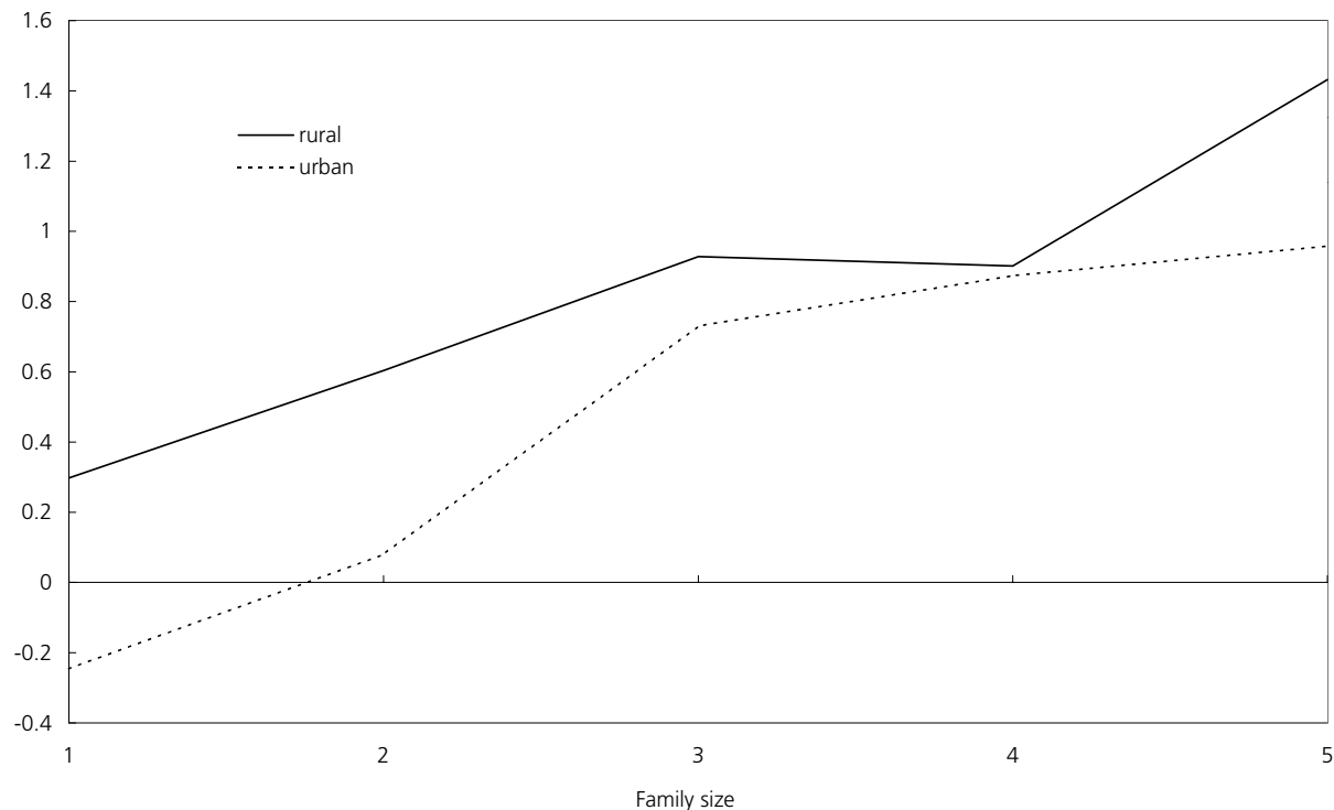
Figure 2 The logit function for the empirical response rate with respect to family size 1, ..., 5 in urban and rural areas, respectively. The computation is based on both the respondents and the nonrespondents from Table A1 in Appendix A
