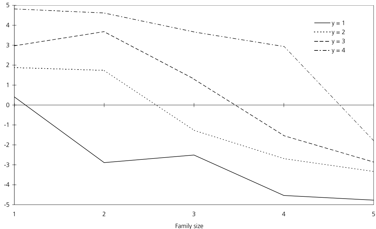
Figure 1. The estimated cumulative logit function, \log\{\hat{P}(Y \leq y | x_1) / (1 - \hat{P}(Y \leq y | x_1))\} , for household sizes 1,..., 4 with respect to family size x_1 . The estimates are based on the free model (3.1) in combination with the response model RM2( y, x_2 )
