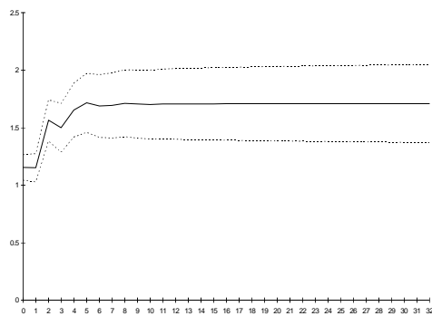
Figure 2. Cumulative impulse response function: Norway price (GDP Deflator)
