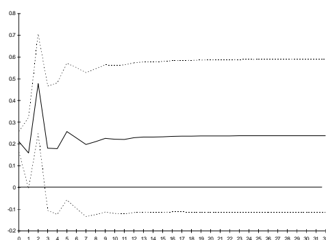
Figure 1. Cumulative impulse response function: Norway Manufacturing Production
