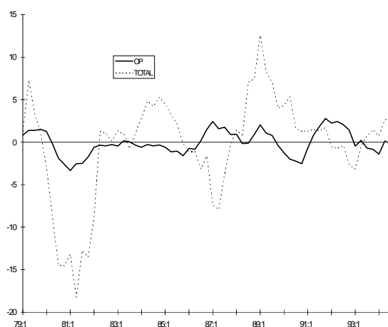
Figure 10. Forecast error decompositions for Manufacturing production in United Kingdom
