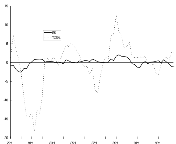
Figure 10. Forecast error decompositions for Manufacturing production in United Kingdom
