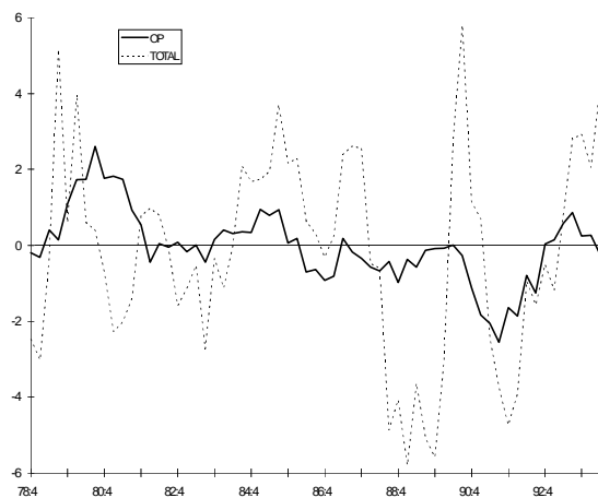
Figure 9. Forecast error decompositions for Manufacturing production in Norway
