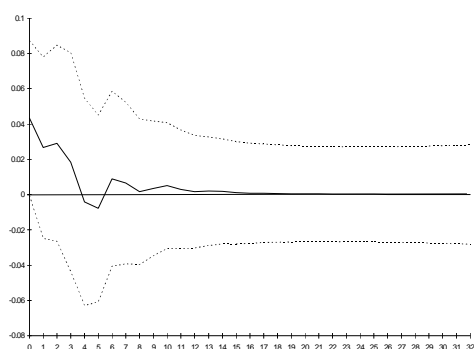
Figure 6. Impulse response functions: Norway Unemployment
