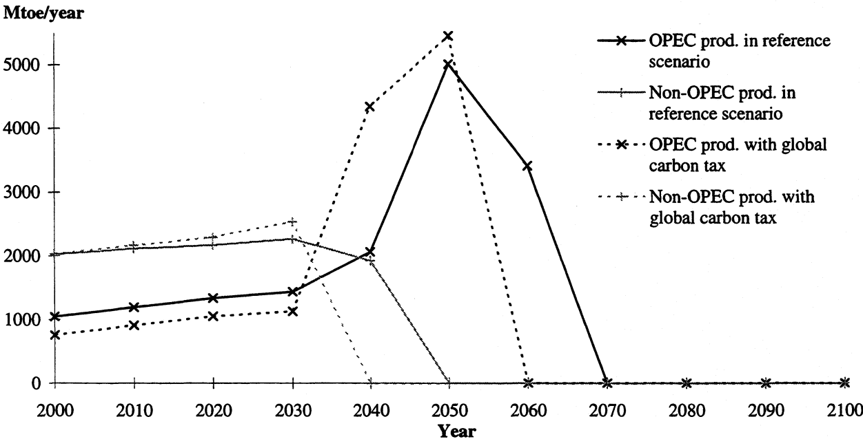
Figure 2. Production of oil in OPEC and Non-OPEC in different scenarios
