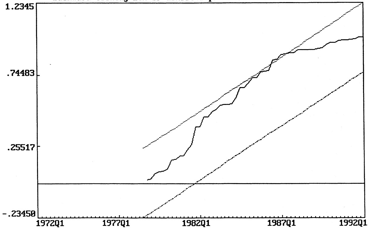
Figure 7: Plot of cumulative sum of squares of recursive residuals (CUSUMQ). Backward looking ECM of domestic prices.
