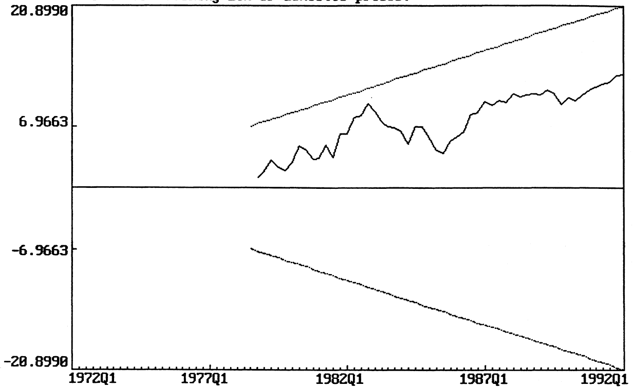
Figure 6: Plot of cumulative sum of recursive residuals (CUSUM). Backward looking ECM of domestic prices.
