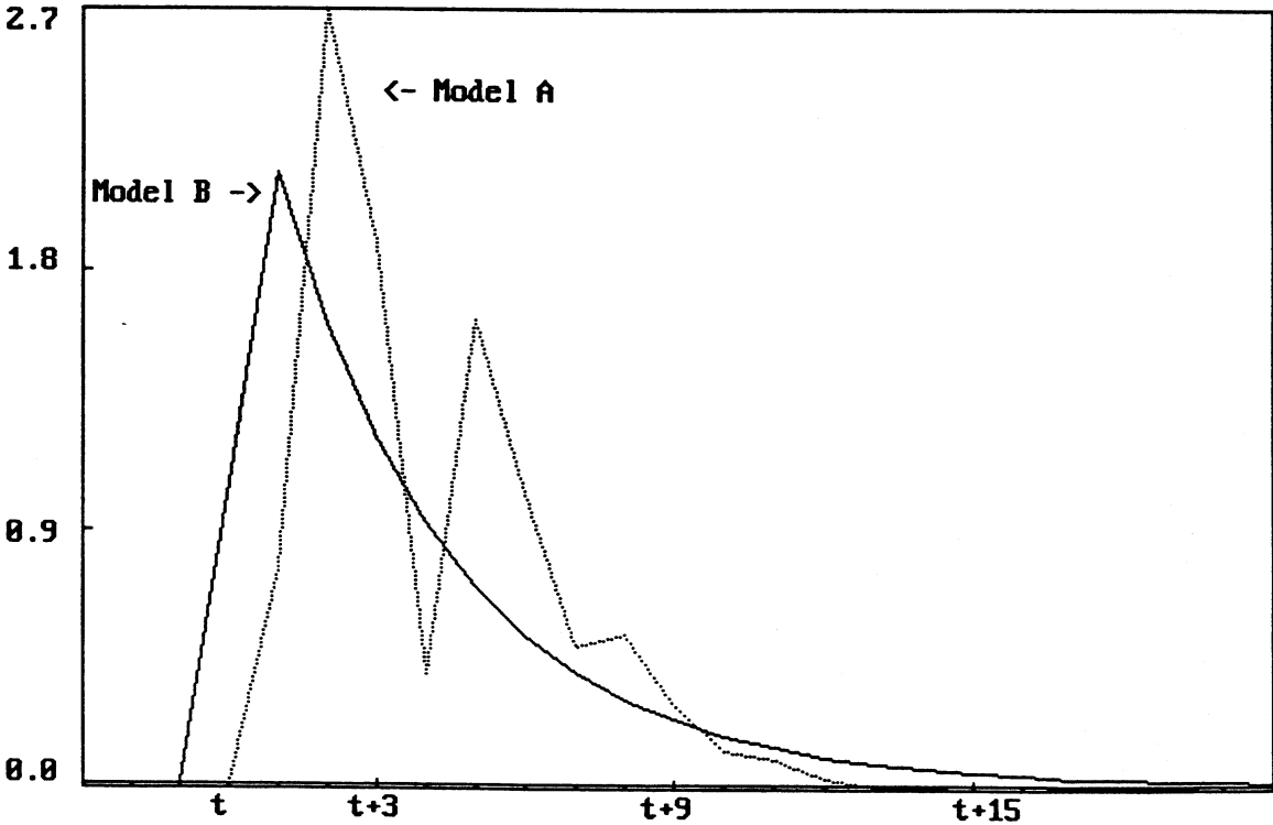
Figure 13: Shock. 10% increase in PW, PK and PE in t.
