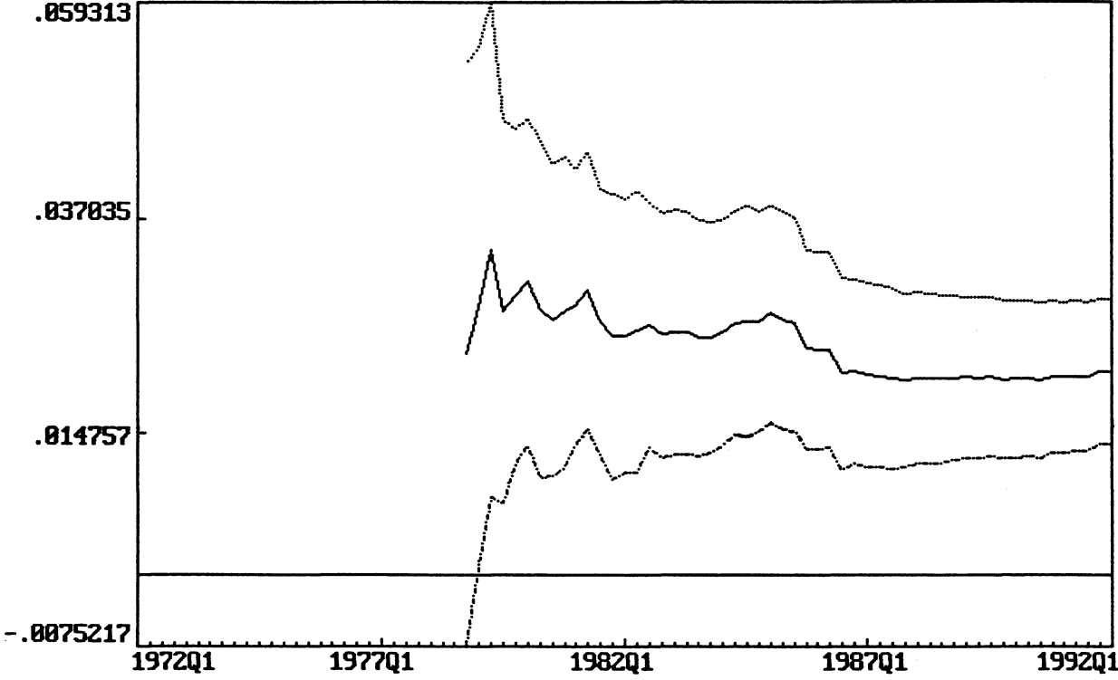
Figure k: Coef. of dk85 \cdot d3 and its 2 S.E. bands based on recursive OLS. Backward looking ECM of domestic prices.
