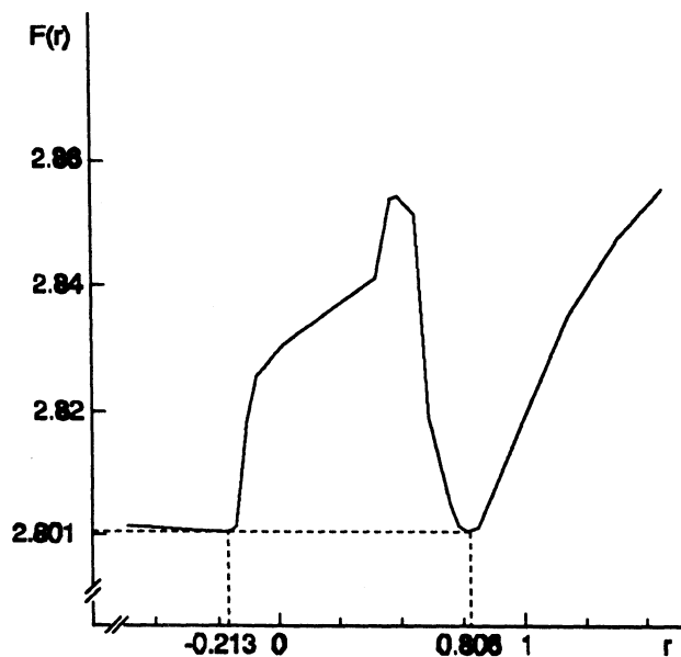
Fig. 2. F-values of M1W3L3 with two solutions
