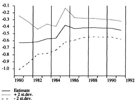
Figure C.12. Recursive estimates - equation (3.16)
