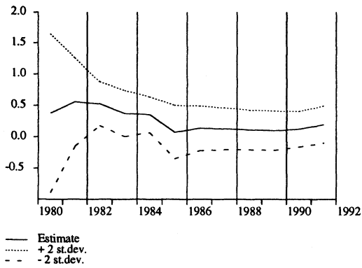
Figure C.7. Recursive estimates - equation (3.16) Coefficient: \beta_1
