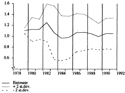
Figure C.1. Recursive estimates - equation (3.13)
