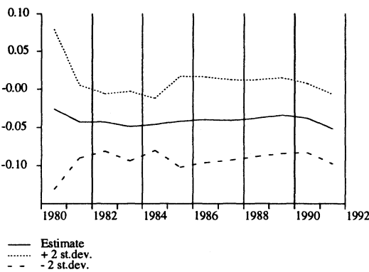
Figure C.8. Recursive estimates - equation (3.16)
