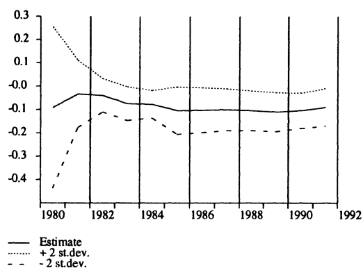
Figure C.13. Recursive estimates - equation (3.16) Coefficient: - beta 7
