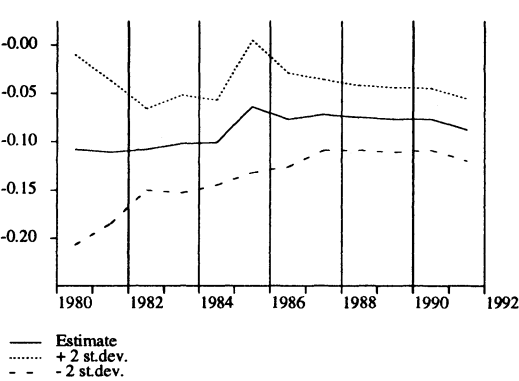
Figure C.10. Recursive estimates - equation (3.16)
