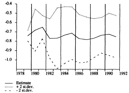
Figure C.2. Recursive estimates - equation (3.13)
