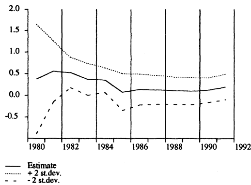
Figure C.7. Recursive estimates - equation (3.16)
