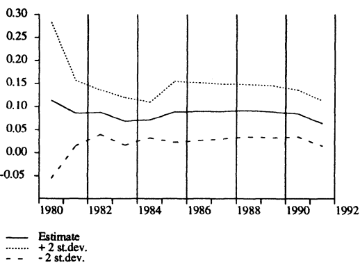
Figure C.9. Recursive estimates - equation (3.16)
