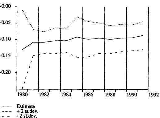
Figure C.11. Recursive estimates - equation (3.16)
