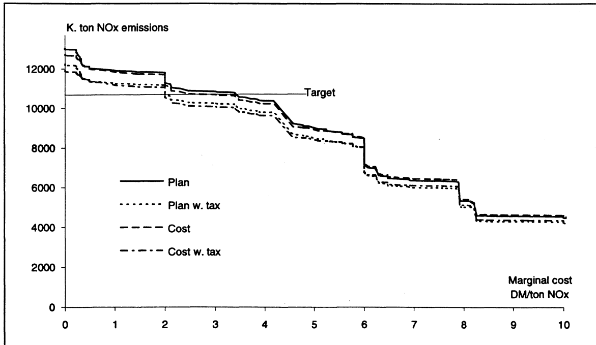
Figure 4a. Marginal NO x abatement costs in the SEEM area. Year 2000
