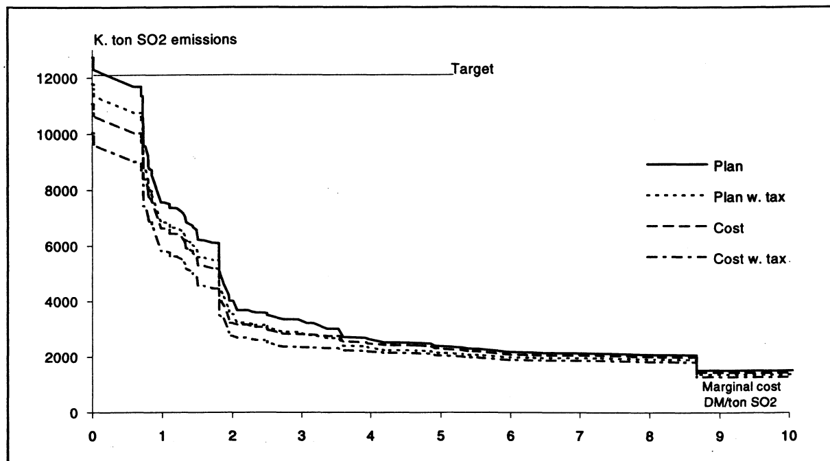
Figure 4b. Marginal SO 2 abatement costs in the SEEM area. Year 2000
