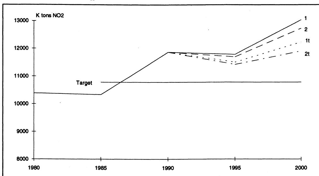
Figure 3b. Simulated \text{NO}_x emissions under both regimes, with and without the EC tax
