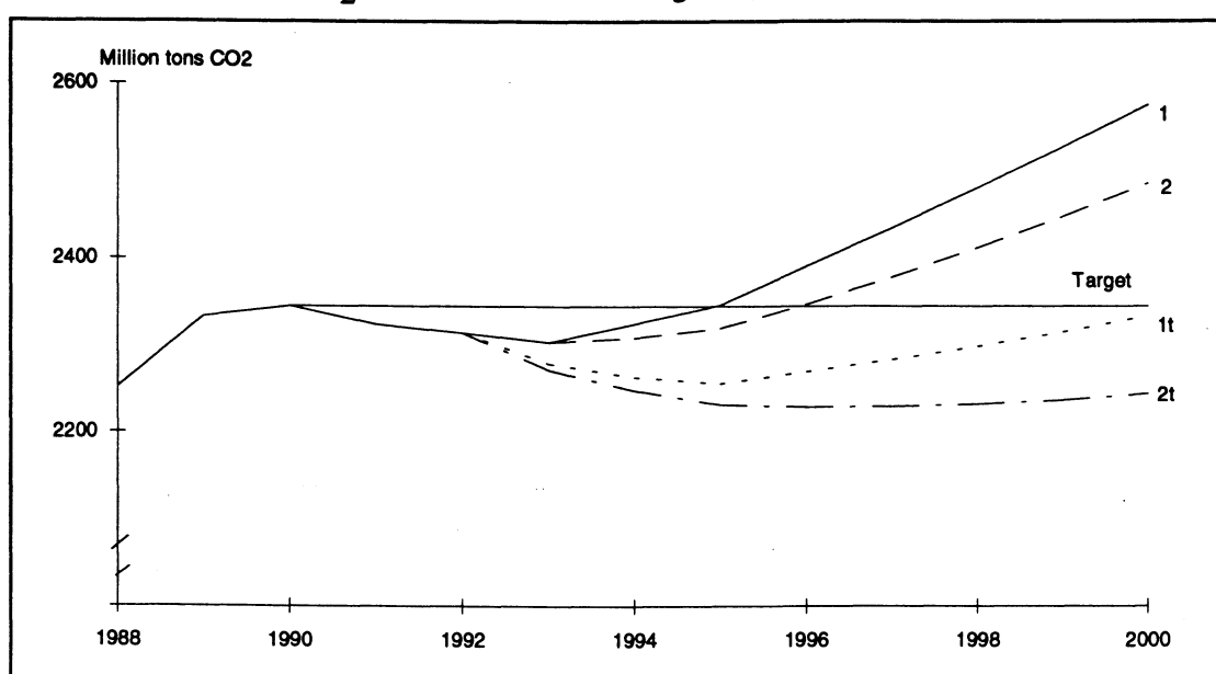
Figure 3a. Simulated \text{CO}_2 emissions under both regimes, with and without the EC tax
