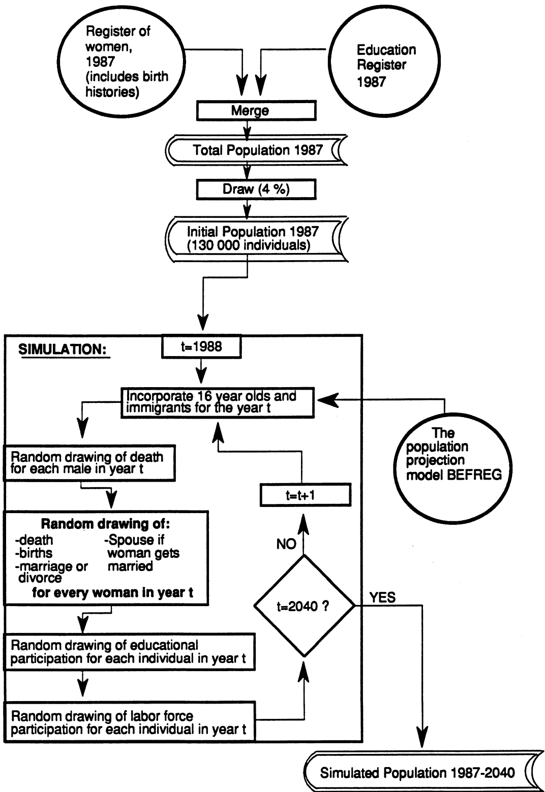
Figure 1. Main structure of MOSART (with exogenous input of 16 year olds)
