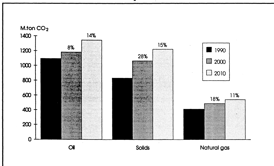
Figure 3.1 CO 2 emissions from solids, oil and natural gas. Reference scenario. 1990, 2000 and 2010. Million metric tons CO 2
