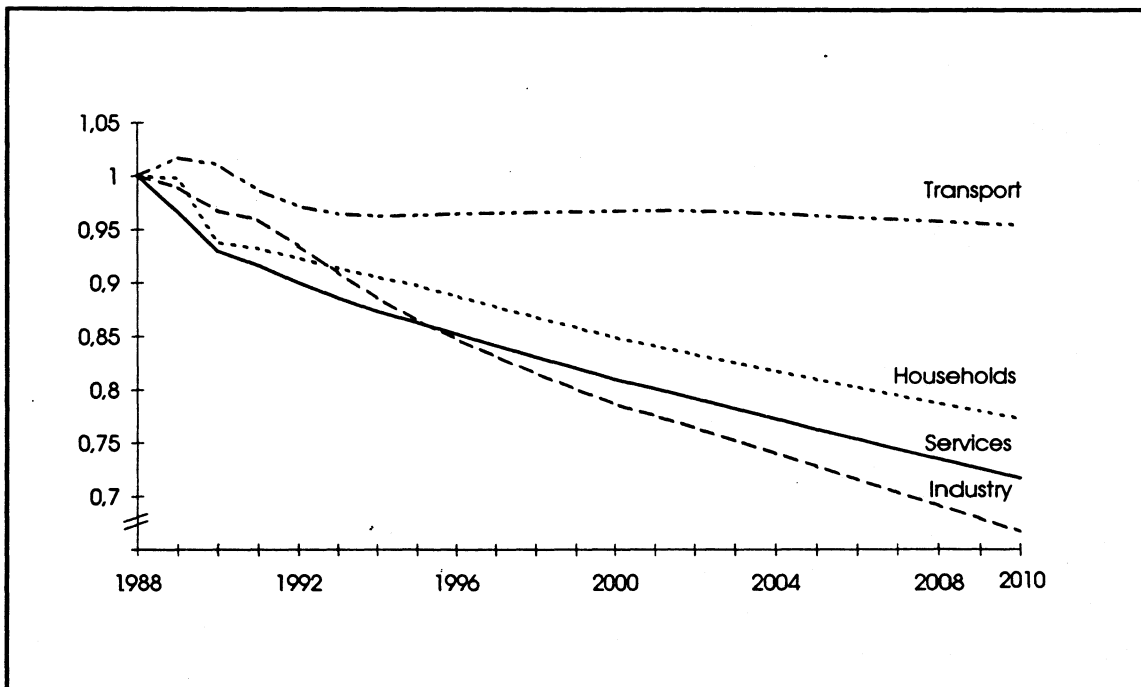
Figure 3.10 Energy intensities by sector. Reference scenario. 1988-2010. Index, 1988=1
