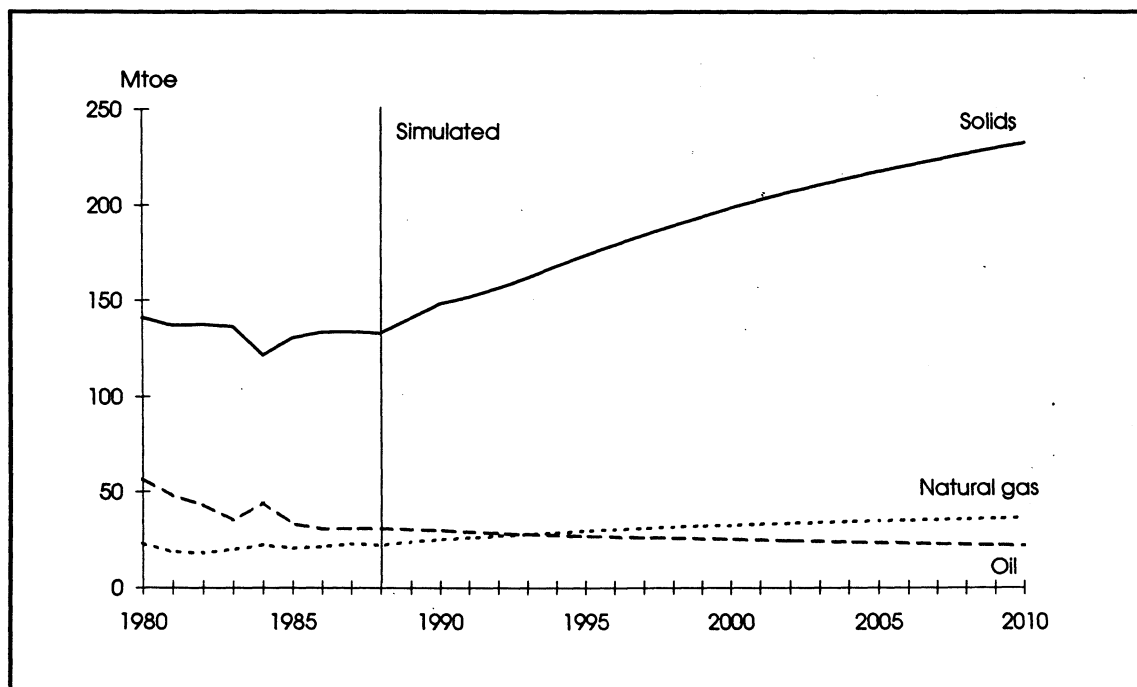
Figure 3.8 Energy demand. Thermal power production. Reference scenario. 1980-2010. Mtoe
