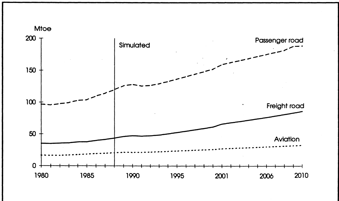
Figure 3.7 Energy demand. Transport. Reference scenario. 1980-2010. Mtoe
