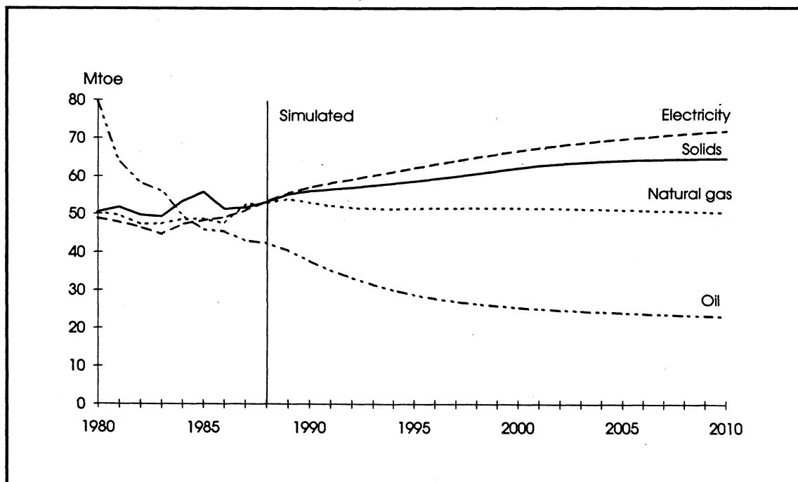
Figure 3.4 Energy demand. Industry. Reference scenario. 1980-2010. Mtoe
