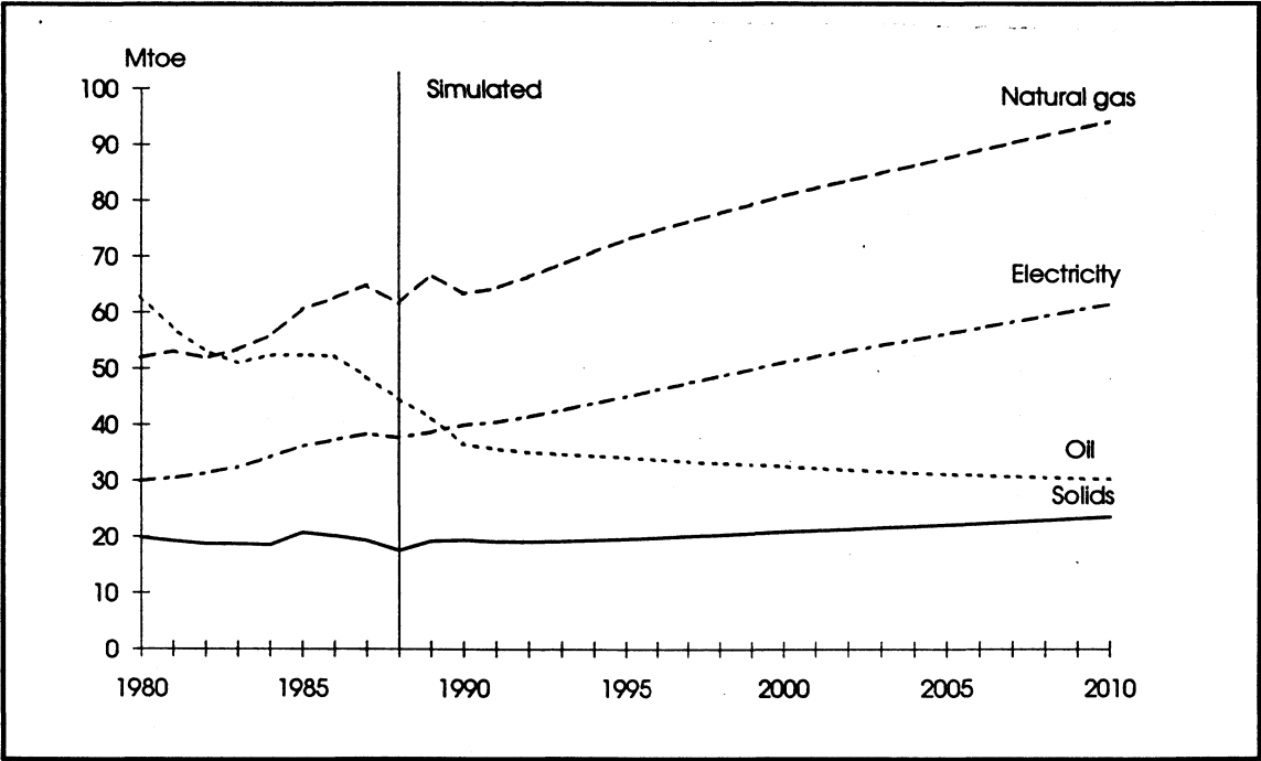
Figure 3.5 Energy demand. Households. Reference scenario. 1980-2010. Mtoe
