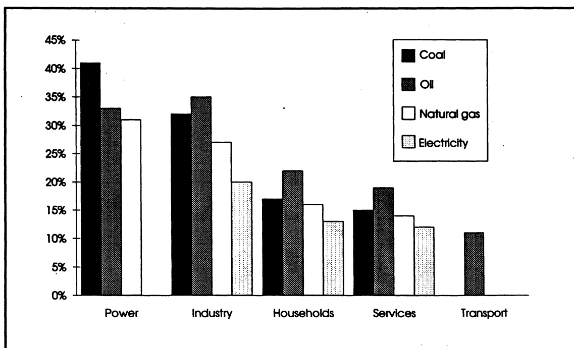
Figure 4.1 Changes in energy prices and demand. Germany (West). EC tax scenario vs. reference scenario. 2000. Per cent
