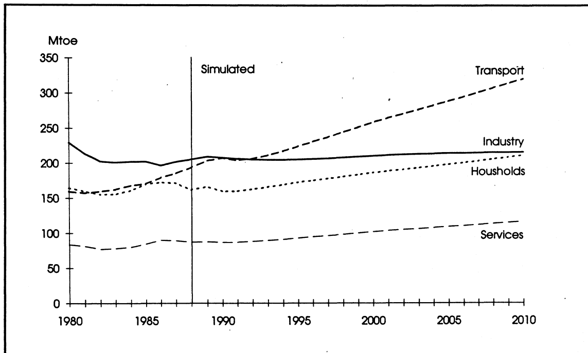
Figure 3.3 Energy end use by sector. Reference scenario. 1980-2010. Mtoe
