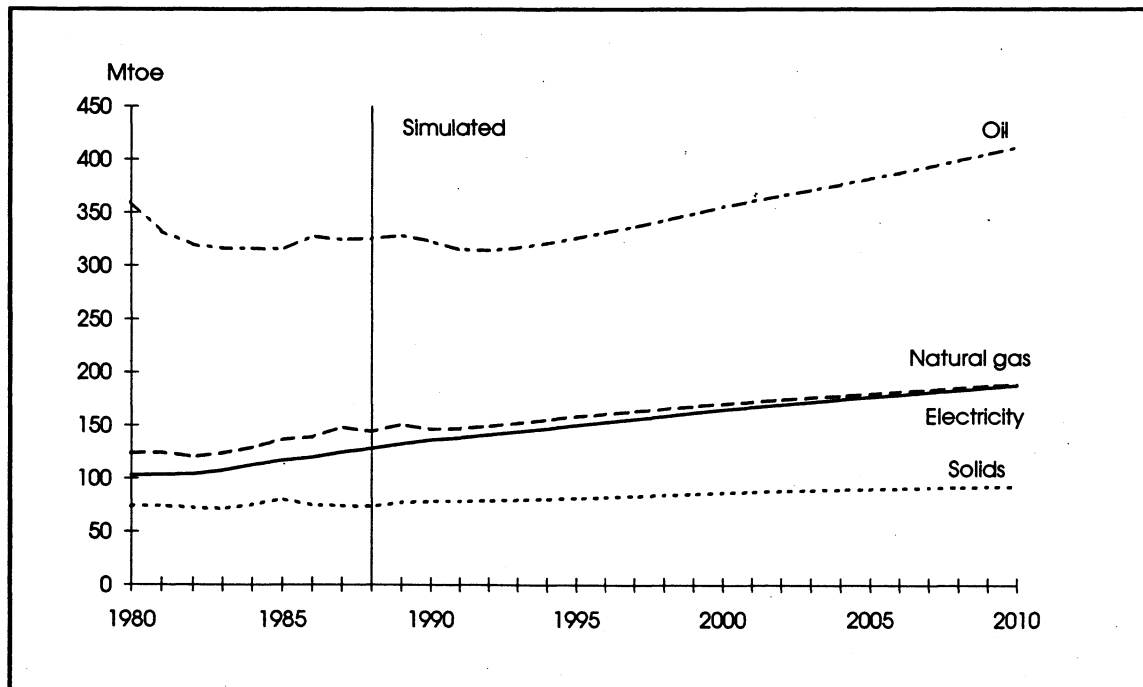
Figure 3.2 Energy end use by fuel. Reference scenario. 1980-2010. Mtoe
