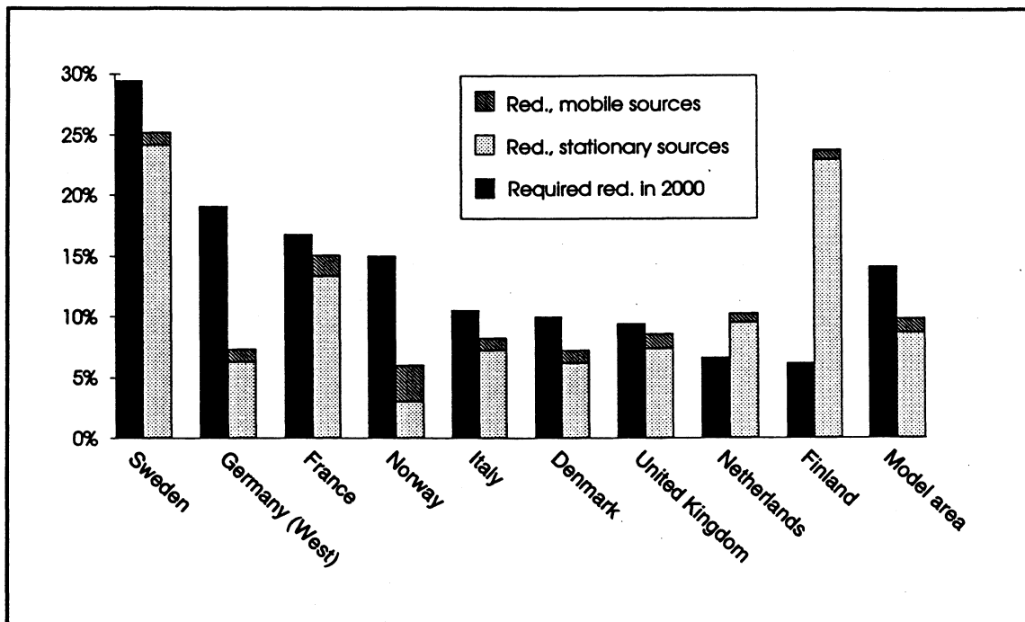
Figure 4.5 Required and simulated reductions in CO 2 emissions by country. EC tax scenario vs. reference scenario. 2000. Per cent
