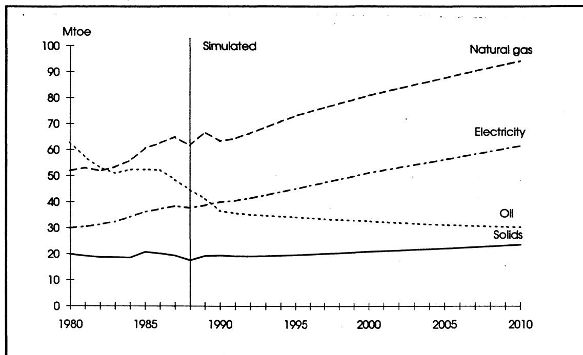
Figure 3.5 Energy demand. Households. Reference scenario. 1980-2010. Mtoe
