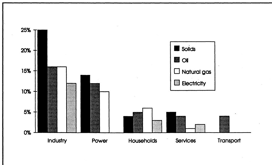
Figure 4.4 Per cent reductions in fuel demand by sector. EC tax scenario vs. reference scenario. 2000
