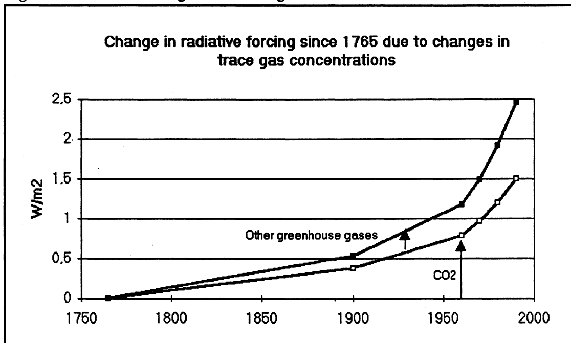
Figure 1 Radiative forcing due to trace gases relative to 1765. Wm^{-2}
