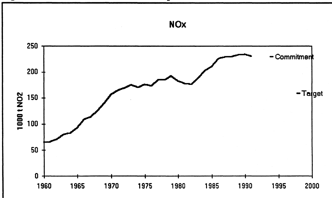
Figure 2 National emissions to air of NO x
