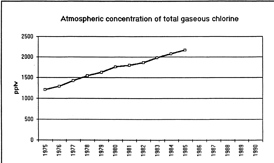
Figure 1 Atmospheric concentration of gaseous chlorine 1975-1985. pptv
