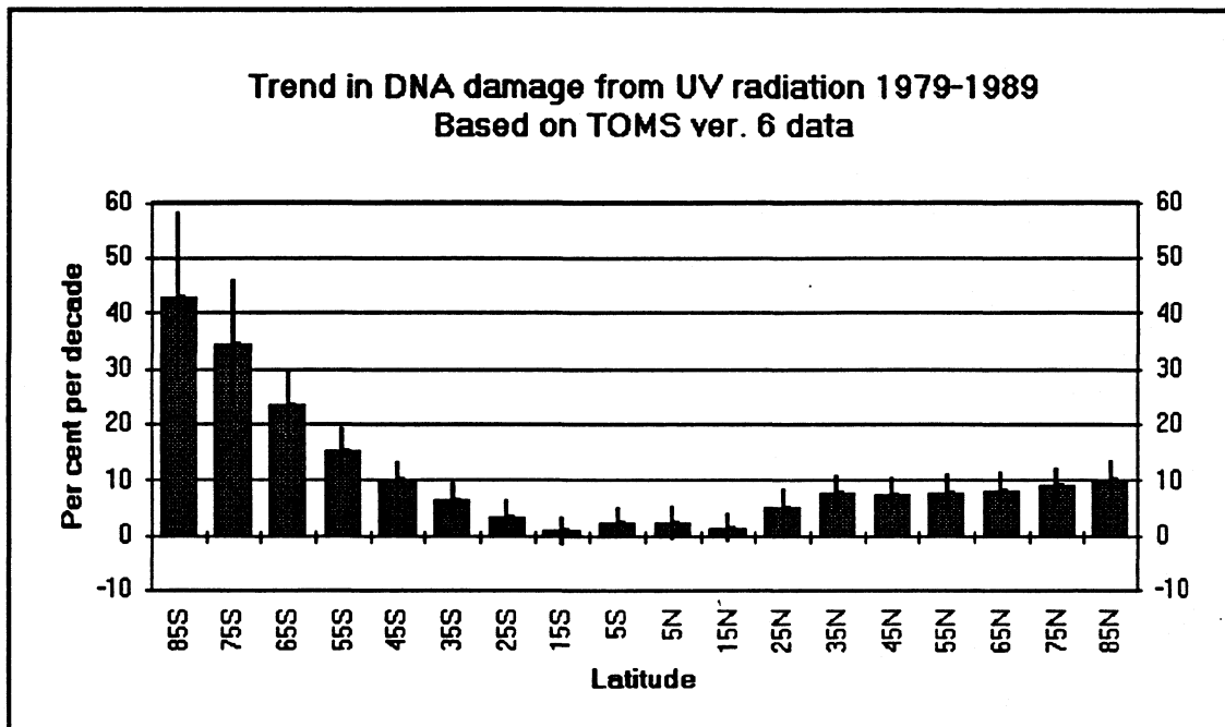
Figure 1 Estimated UV damage to DNA due to depletion of the ozone layer, 1979-1989
