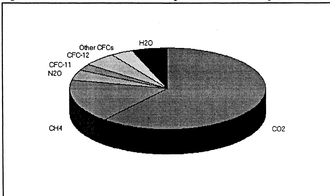
Figure 2: Contribution from different trace gases to radiative forcing in 1990
