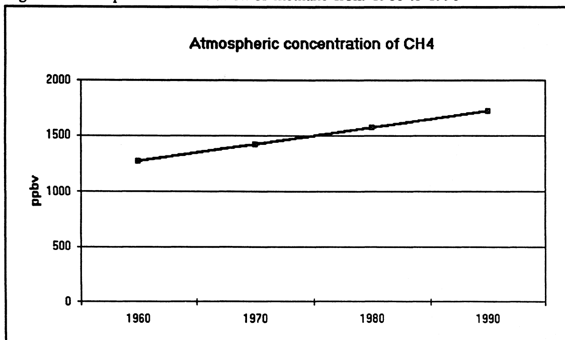
Figure 4 Atmospheric concentration of methane from 1960 to 1990
