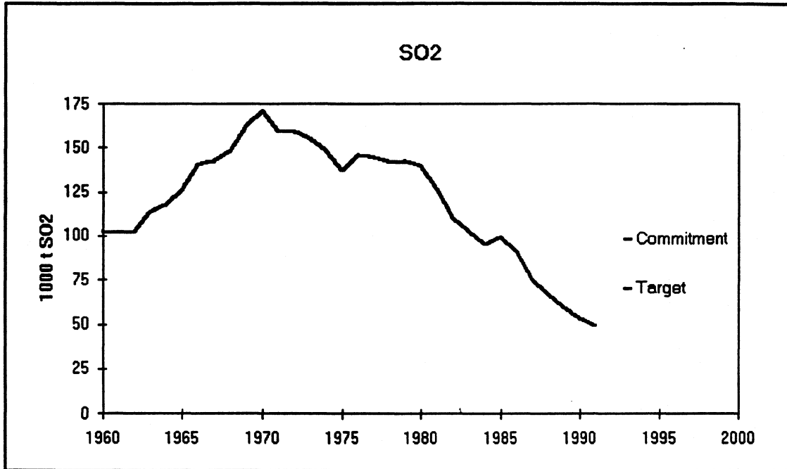
Figure 1 National emissions to air of SO 2
