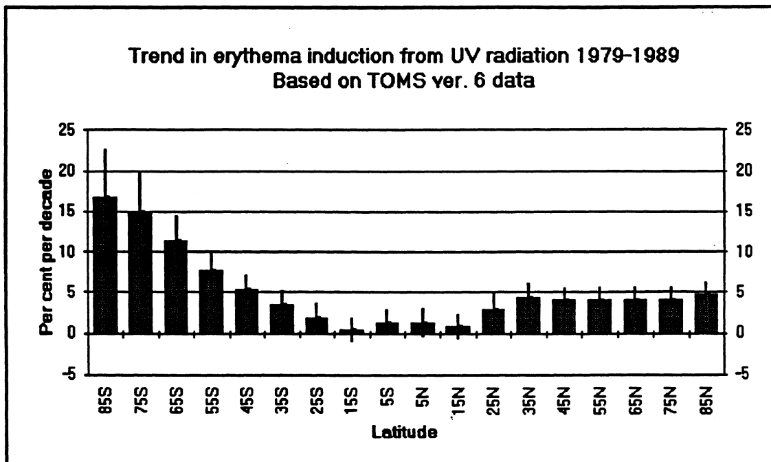
Figure 3 Estimated UV damage to skin due to depletion of the ozone layer. 1979-1989
