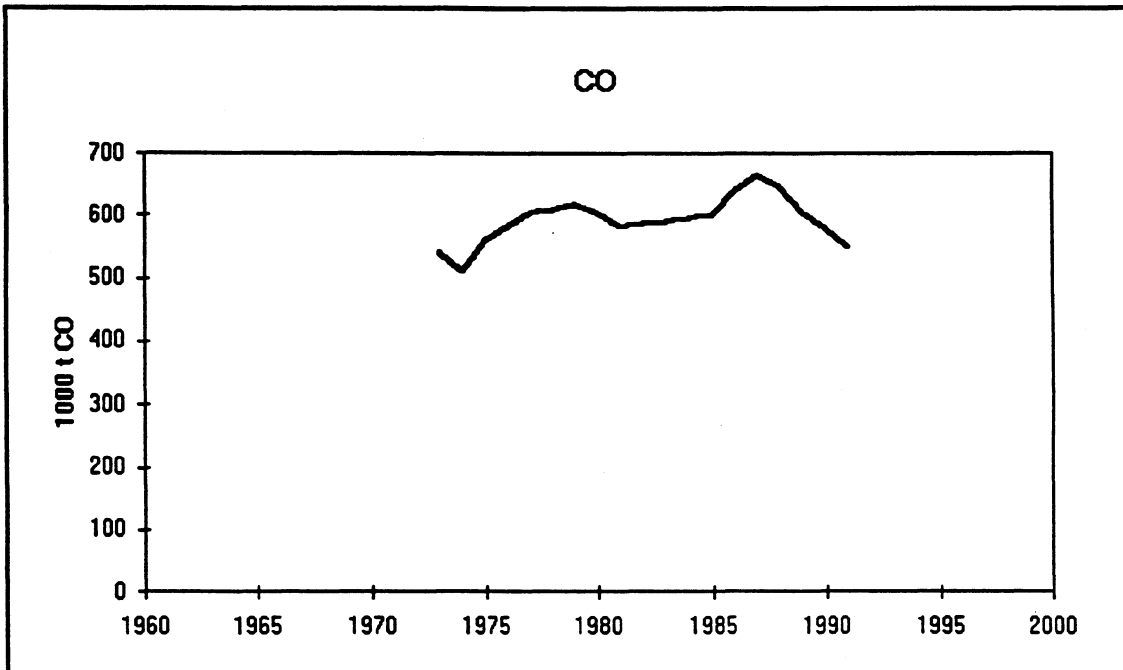
Figure 4 National emissions to air of CO
