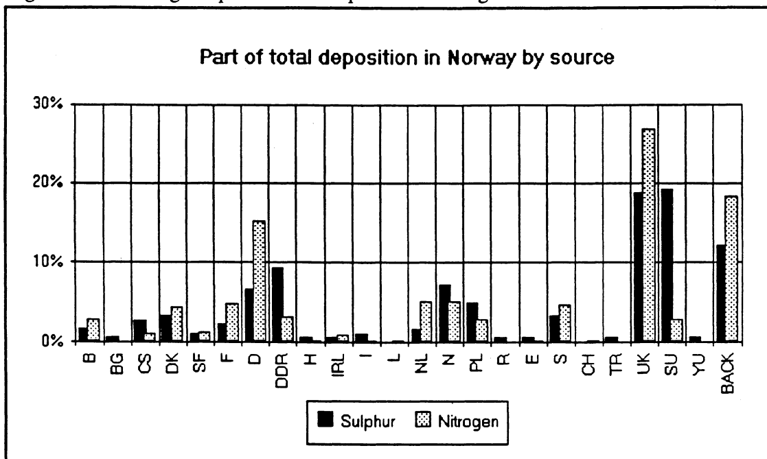
Figure 1 Percentage deposition of sulphur and nitrogen from different sources
