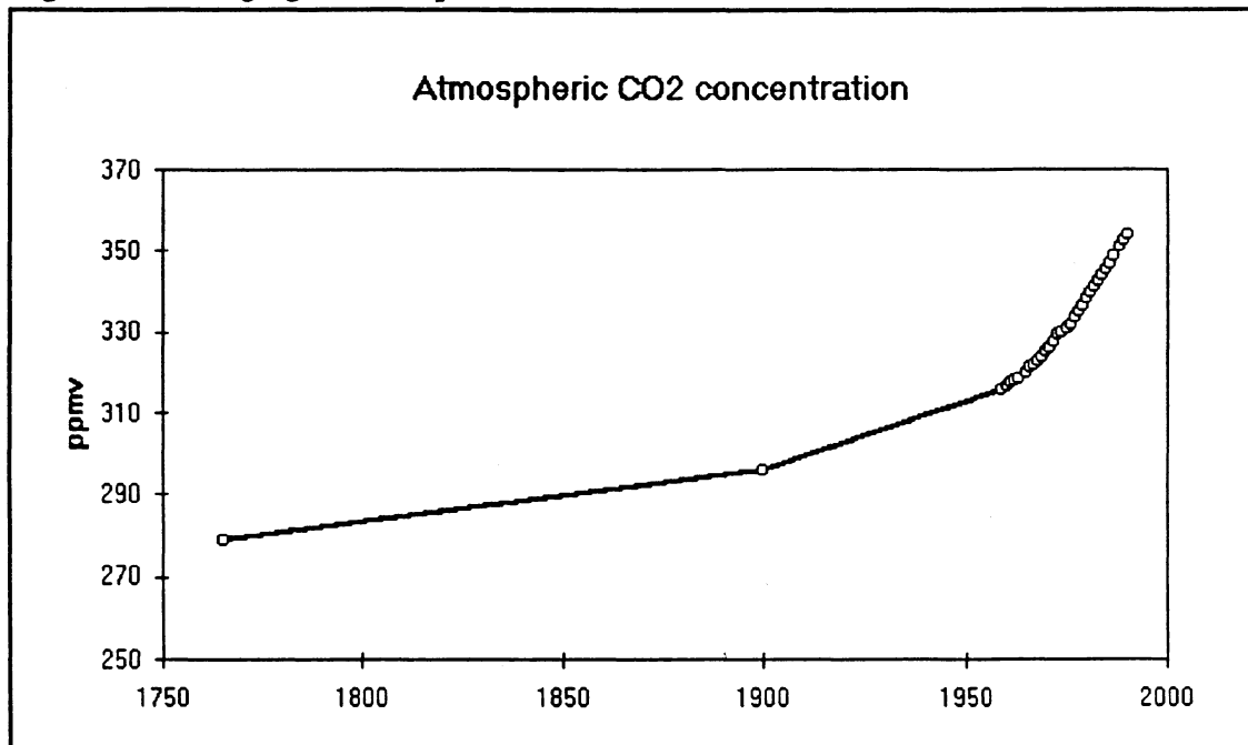
Figure 1 Average global CO 2 concentration 1765-1990.
