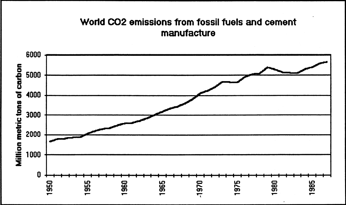
Figure 5 Global CO 2 emissions from fossil fuels and cement manufacture 1950 - 1987
