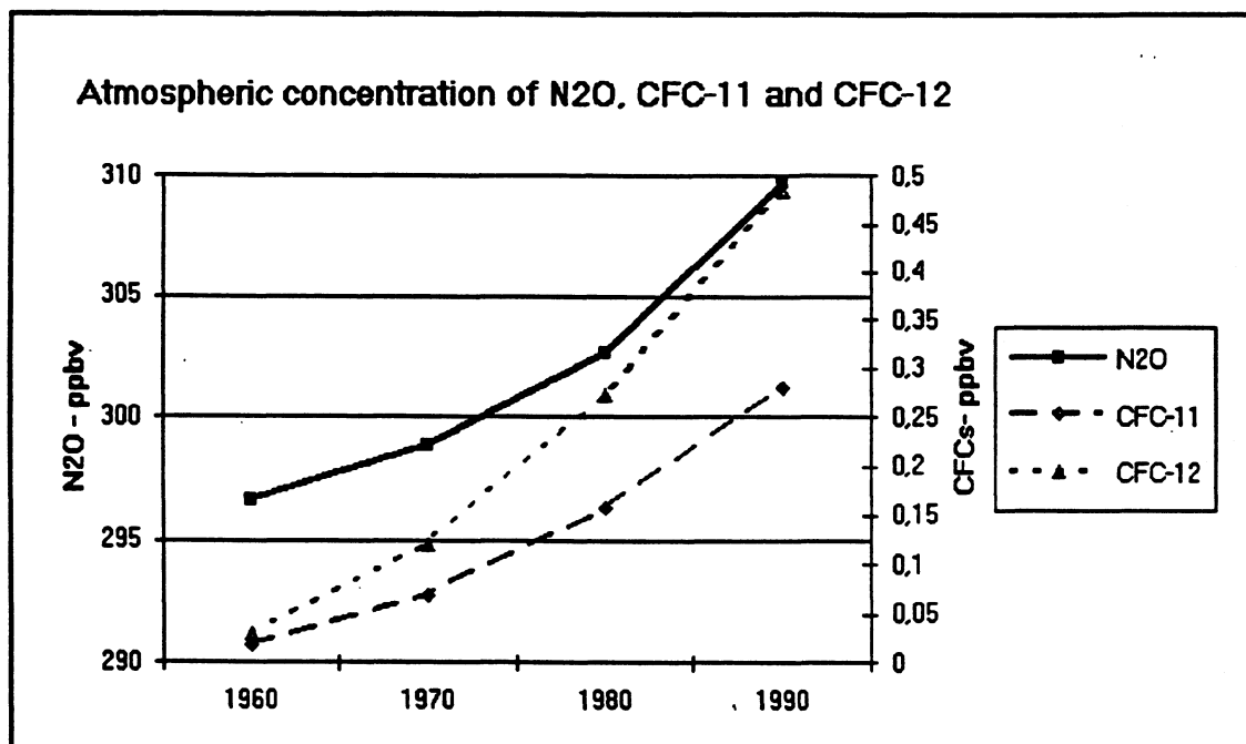
Figure 3 Atmospheric concentration of nitrous oxide, CFC-11 and CFC-12 from 1960 to 1990
