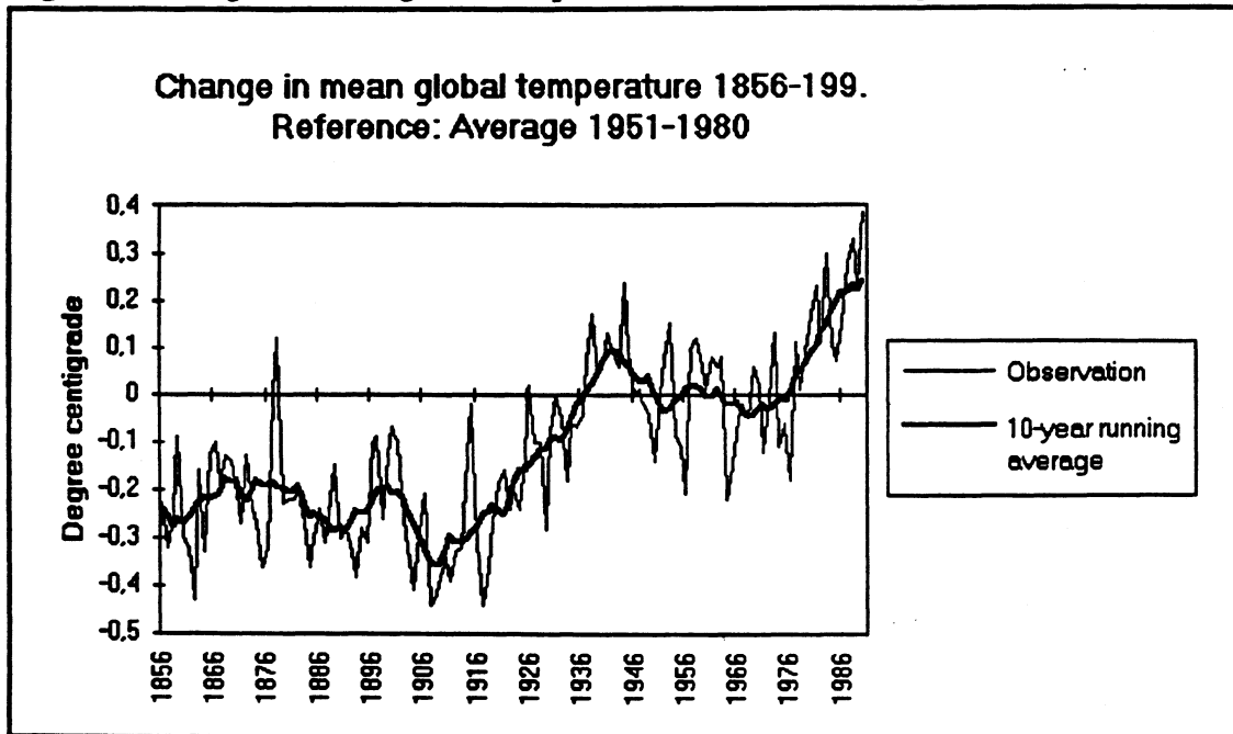
Figure 1 Change in mean global temperature relative to average 1951-1980...
