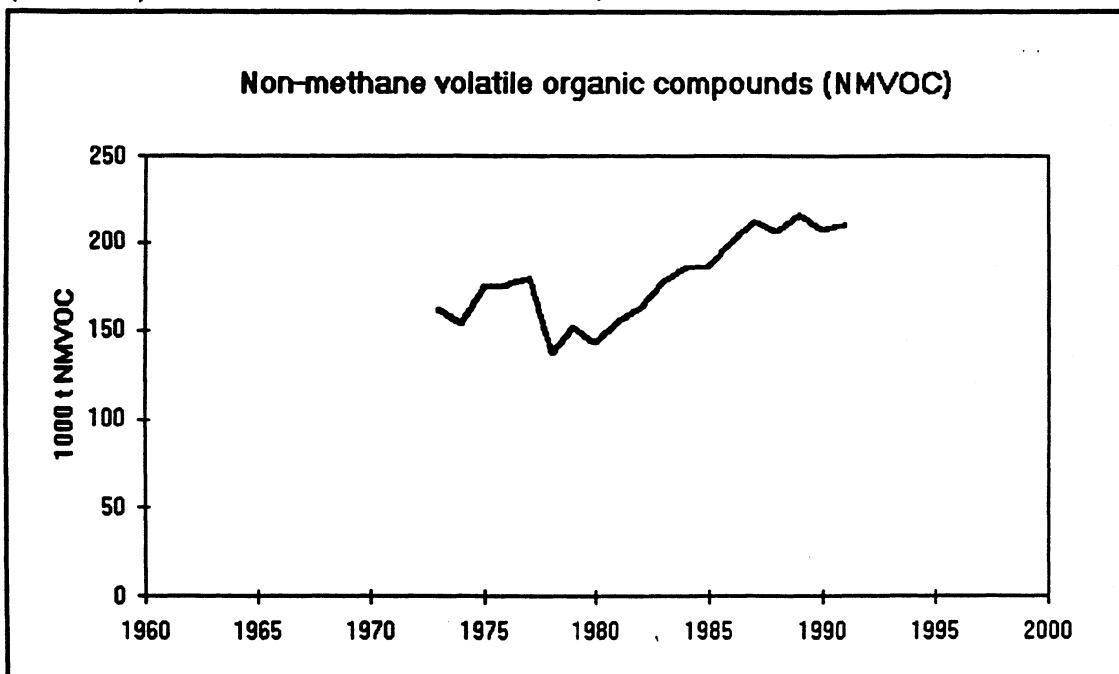
Figure 7 National emissions to air of non-methane volatile organic compounds (NMVOC)
