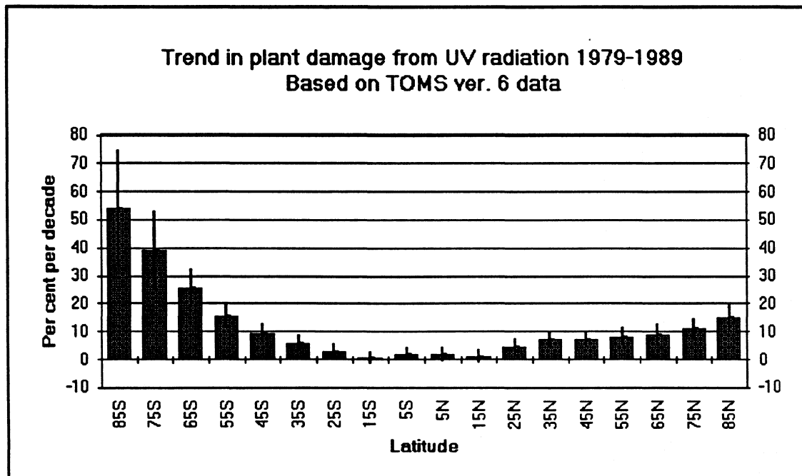
Figure 2 Estimated UV damage to plants due to depletion of the ozone layer, 1979-1989
