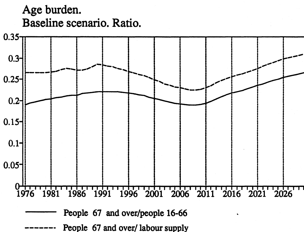
Fig 7. Age burden
