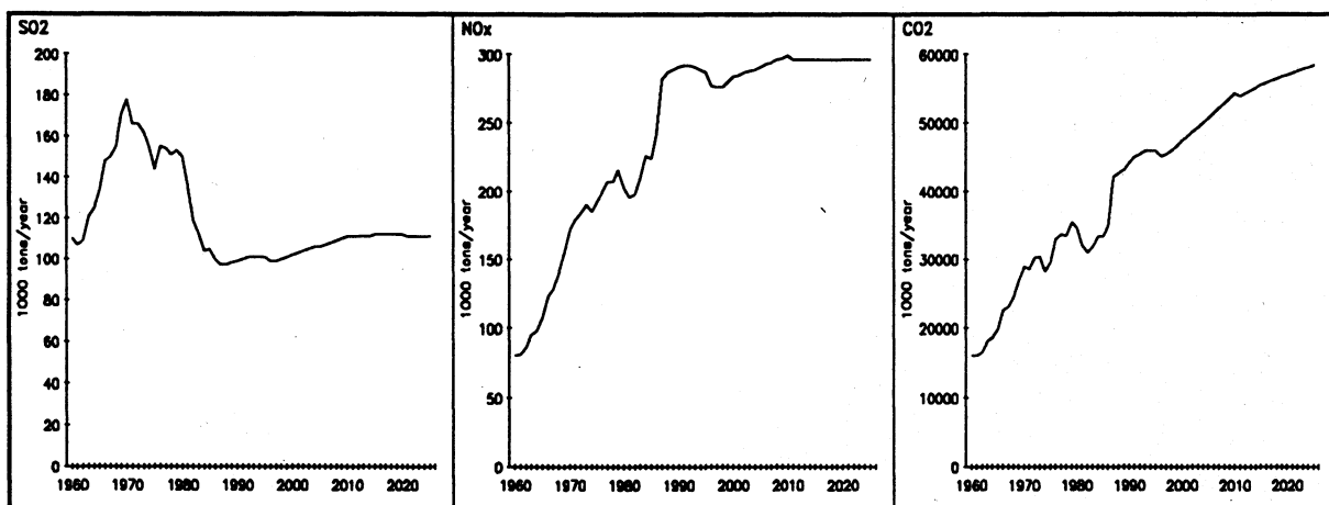
Figure 1 Emission projections
