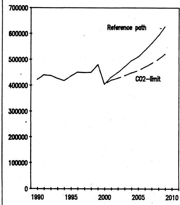
Figure 7. CO emissions. 1990–2010
