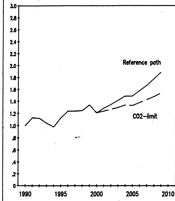
Figure 6. SO 2 emissions. 1990–2010
