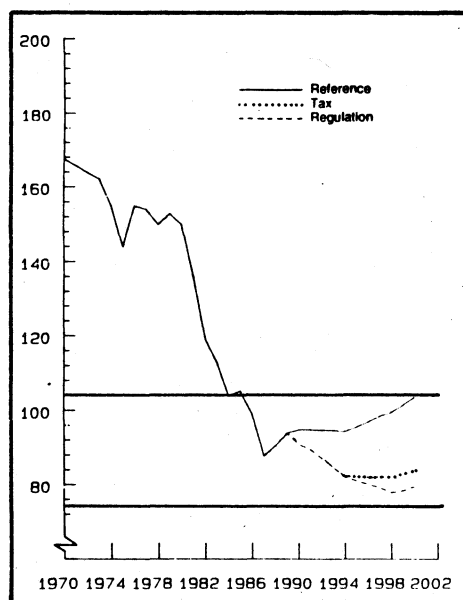
Figure 5.5.1. Emissions of SO_2 . 1000 metric tons per year. 1970-2000
