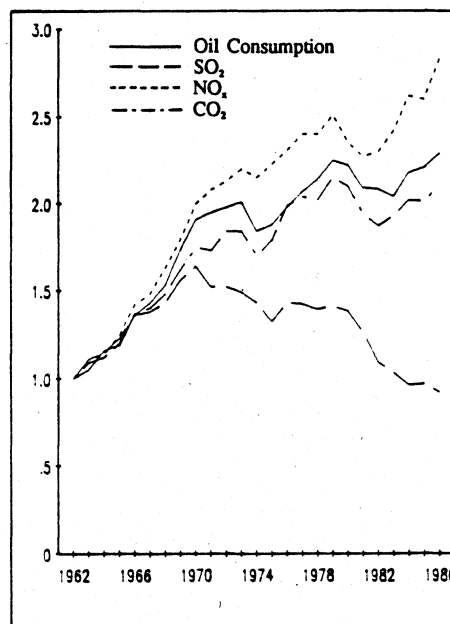
Figure 2.6. Consumption of Oil Products and Emission of SO_2 , NO_x and CO_2 . Norway. 1962-1986. Indices, 1962=1
