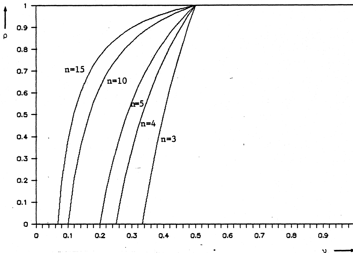
Figure 1: The T(\nu, \rho; n)=0 lines for different values of n
