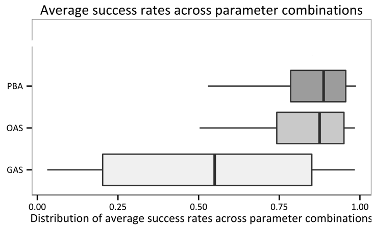
FIGURE B.2. Distribution of average success rates, p = \mathbb{E}[\mathcal{S}]
