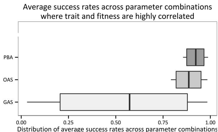
FIGURE B.3. Distribution of average success rates, p = \mathbb{E}[\mathcal{S}] , if correlation is high
