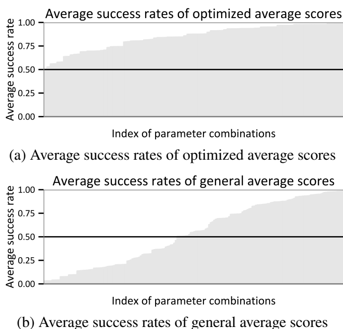
FIGURE B.4. Recommendation success of average scores
