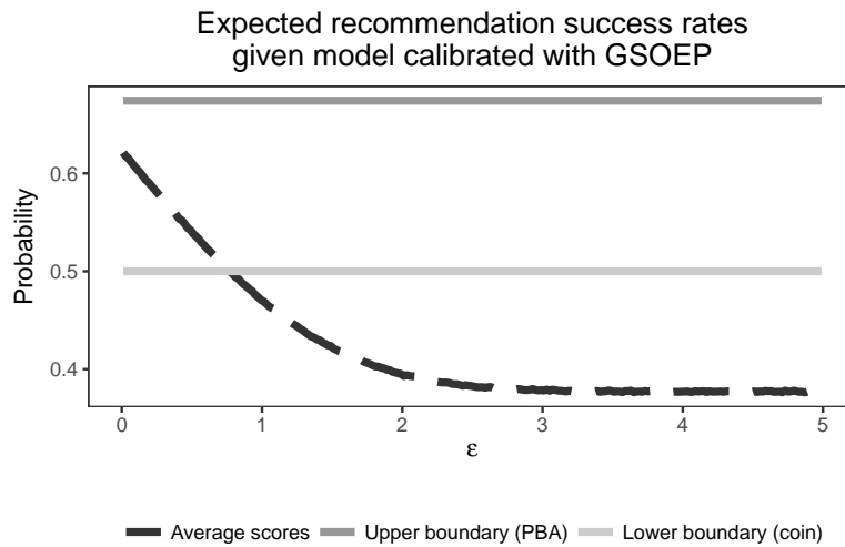
FIGURE 2. Expected recommendation success using model calibrated with SOEP data
