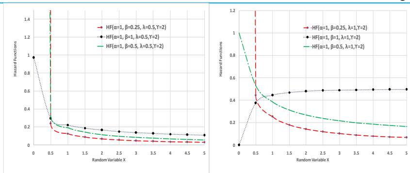
Figure 2a: Hazard Function for the Weibull- Weibull-Burr III ( \alpha , \lambda and \gamma = shape and \beta= scale parameters)
