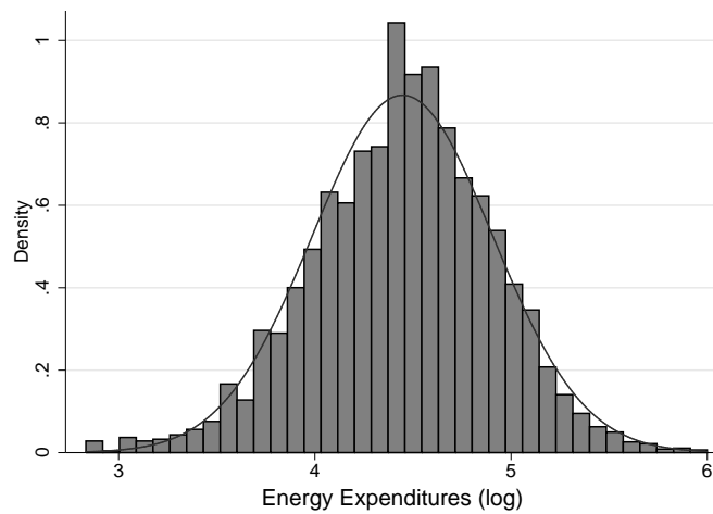
Figure 2: Histogram for household energy expenditures, overlaid with best-fit Gaussian density (fitted to empirical mean and standard deviation).
