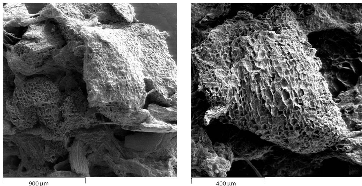
Figure 1: Scanning electron microscope images of cork granules embedded in faecal matrix (left) and recovered from the sludge box (right) (Unger et al. 2015, 230p).
