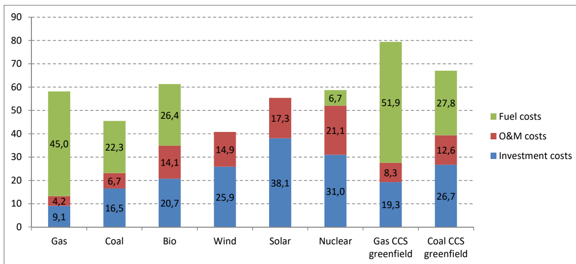
Figure 2 Costs of new electricity in 2030 (€2009/MWh)
