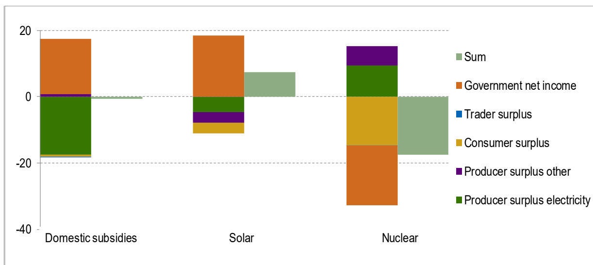
Figure 13 Change in welfare components relative to reference scenario. EU-30 in 2030 (Millions €2009)
