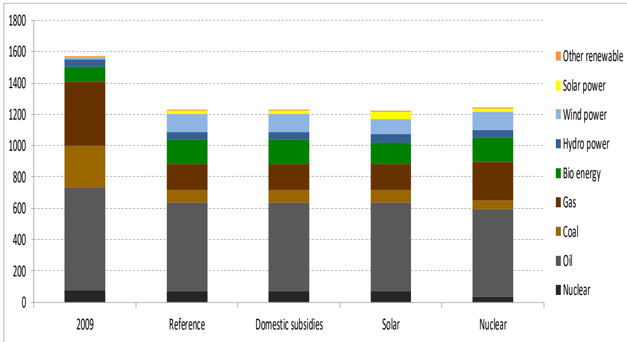
Figure 8 Energy consumption in EU-30 in 2009 and 2030 (Mtoe)
