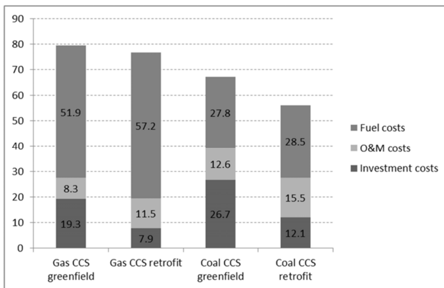
Figure 3 Costs of CCS electricity in 2030 (€2009/MWh)
