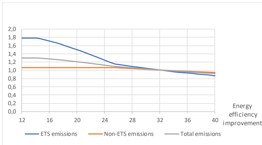
Figure 11 Sensitivity of energy-efficiency target – emissions
